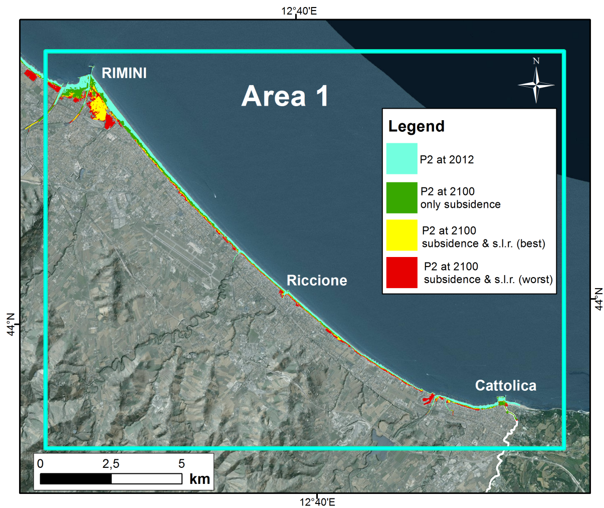
Figure 6. Floodable regions across Area 1 in case of storm surge for case P2 at 2100. The assumptions in modelling are color-coded in the inset. In Figures 6-10 “best” and “worst” refer to the LOW-END and HIGH-END scenarios described in the body of the paper, respectively
