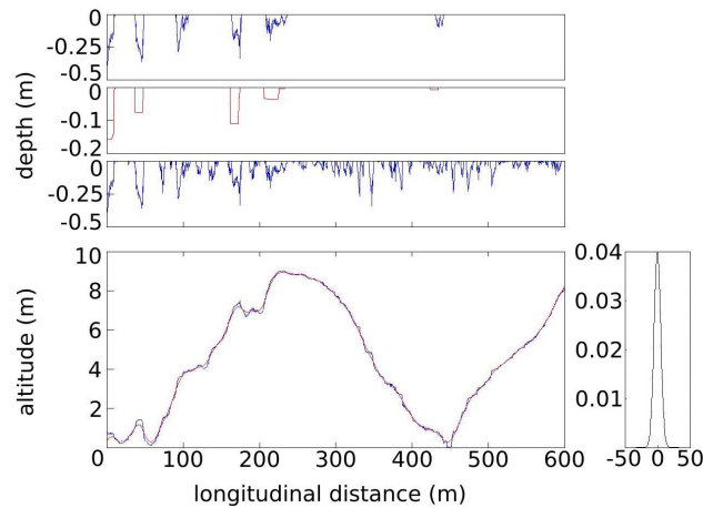
Figure 4. Principle of gullies contour detection. Right: the gaussian filter with 10m standard deviation. Left, from bottom to top: original (blue) and smoothed (red) topography ; raw negative differences between original and smoothed topography ; detection of possible gullies with a threshold on the depth-volume of the element ; detected gullies
