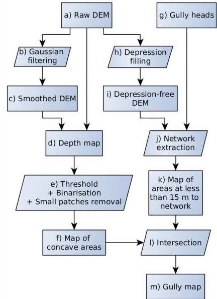
Figure 3. Flowchart of the method used to map gullies from the kite DEM. Letters associated with each step are referenced in the text describing the method in section 2.5
