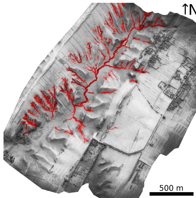
Figure 9. Raw Final result of the proposed gully detection algorithm
