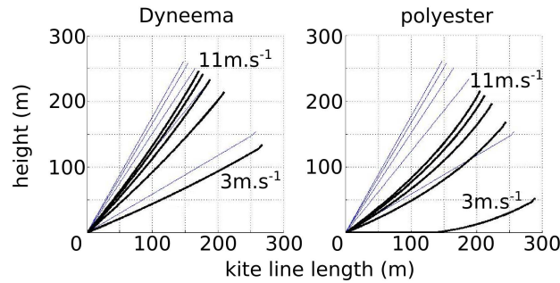
Figure 5. Comparison of the shape of 300m-300 m lines (black bold) with "ideal" (thin grey) ones on a kite flown under different wind conditions. Total load of the rig (Figure 2 - right) for the simulation is 500 g. "Ideal" lines are modelled as weightless and causing no drag. Left: Dyneema® line (0.1 g.m -1 ). Right: polyester line (1 g.m -1 ).
