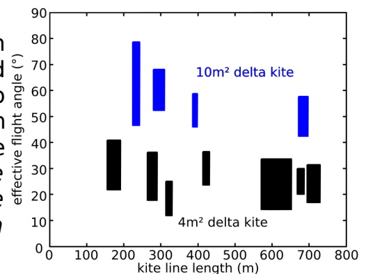
Figure 7. Observed flight angle for the two kites and various conditions of wind speed and line length.
