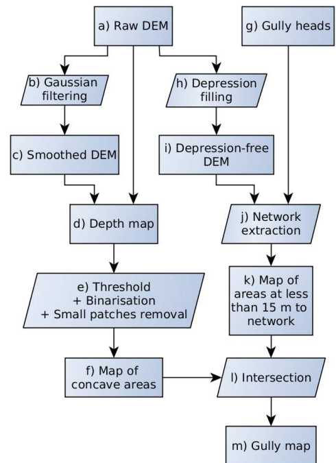
35 Figure 3. Flowchart of the method used to map gullies from the kite DEM. Letters associated with each step are referenced in the text describing the method in section 2.5
