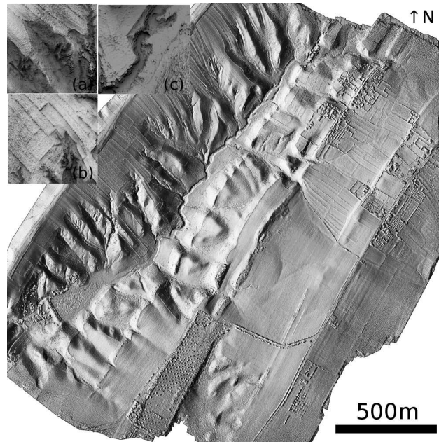
Figure 8. Shaded view views of the computed DEM over the Kamech test site. The main view is a classical shading of the DEM computed with a unique illumination source located east. The three zoomed views are shaded view computed as the portion of visible sky at each point. This type of shading highlights local features such as steep slopes and hard cuts: (a) shows a gully head ; (b) shows some cultivated plots with the plot borders easily visible and a gully head downstream the plots ; (c) shows erosion which grows upstream - regressive erosion - in the main thalweg
