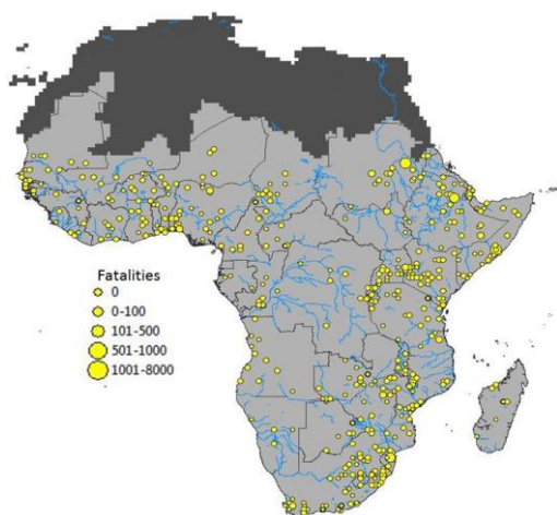
15 Figure 4 Reported flood events (1980-2010) in sub-Saharan Africa grouped per country. The size of the dots shows the number of fatalities that each flood caused (Munich Re, 2014)
