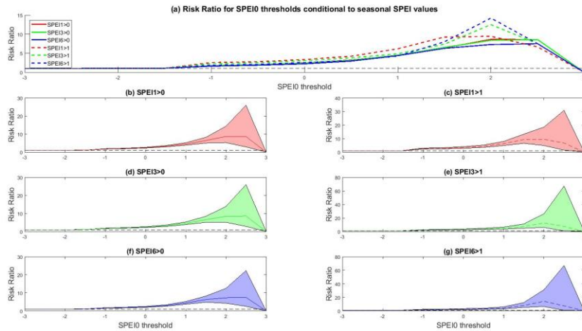
5 Figure 8 Risk ratio between F and NF for given SPEI0 thresholds conditional to seasonal SPEI values (SPEI1>0-red solid, SPEI1>1-red dashed, SPEI3>0-green solid, SPEI3>1-green dashed, SPEI6>0-blue solid, SPEI6>1-blue dashed) (a) and their confidence intervals are shown (b-g). The horizontal dashed line shows the risk ratio of 1.
