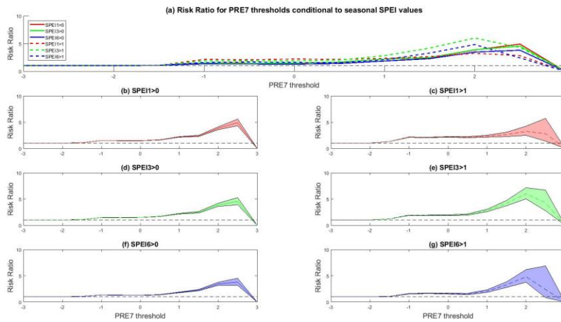
Figure 9 Risk ratio between F and NF for given PRE7 thresholds conditional to seasonal SPEI values (SPEI1>0-red solid, SPEI1>1-red dashed, SPEI3>0-green solid, SPEI3>1-green dashed, SPEI6>0-blue solid, SPEI6>1-blue dashed) (a) and their confidence intervals are shown (b-g). The horizontal dashed line shows the risk ratio of 1.
