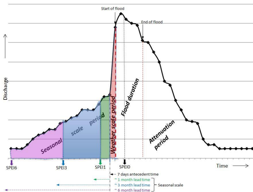
Figure 3: Theoretical discharge before, during and after a hypothetical flood event. Weather scale period starts 7 days before flood onset date. Seasonal scale period is split into 1-, 3- and 6-month accumulation periods. It starts 6 months before flood onset date and continues until the last month before the one that includes the 7-day precipitation. SPEI0 is defined as the SPEI over the calendar month in which the flood onset took place.
