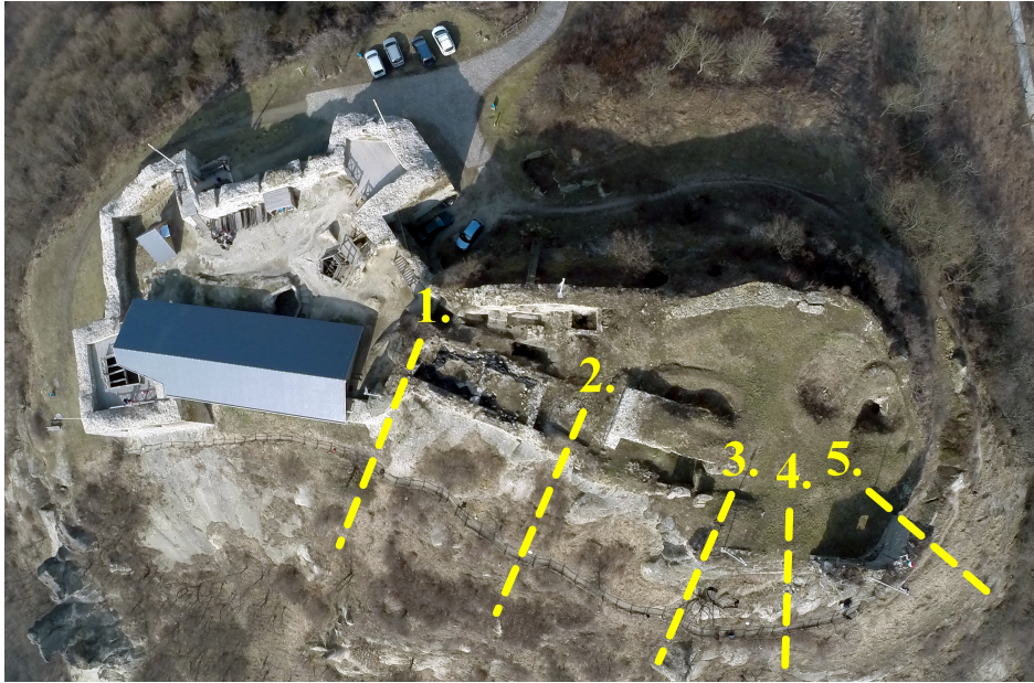
Fig. 1. New Figure, Fig. 14 Location of some studied cross sections
