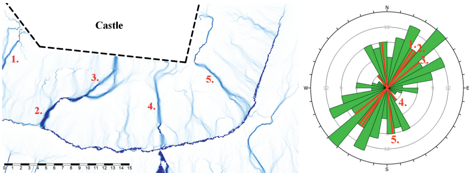
Fig. 2. New Figure: Fig. 12. Joint system obtained by RPAS (marked on catchment area DEM) and also measured on the field. Numbers refer to major joint systems marked on DEM map and on rose diagram
