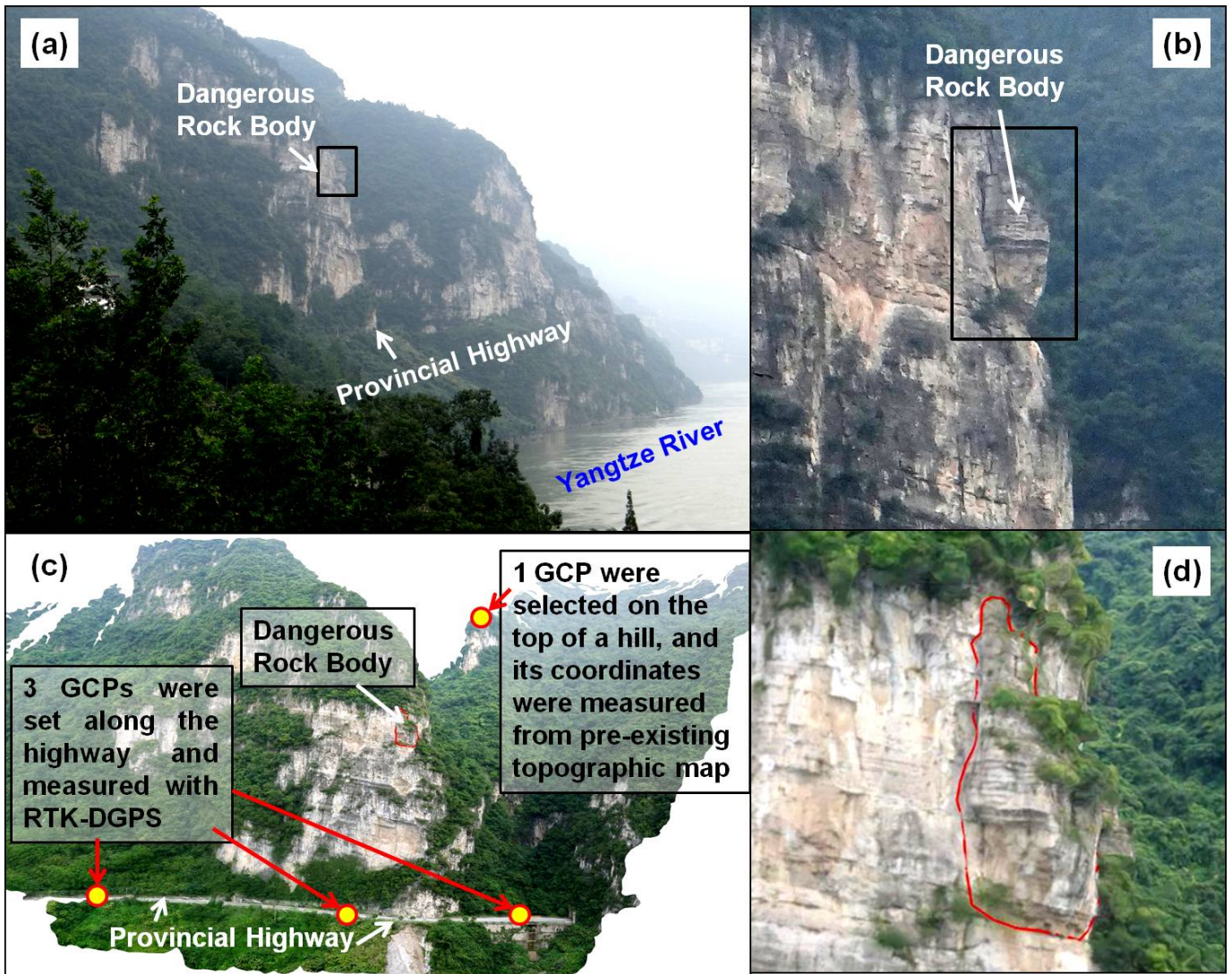
780 Fig.7. The results of a UAV-based emergency investigation for a dangerous rock mass on steep cliff. (a) Overview photo; (b) right side photo of the dangerous rock mass; (c) 3D texture model of the whole scene; (d) 3D texture model of the dangerous rock mass.
