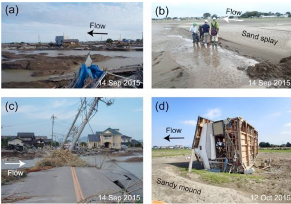
Figure 9: Photos of the study area. (a) Crevasse channel (breach scouring) near the levee. Note the building still standing after the flood in the center of the photo. (b) Sand splay in the southern part of the study area. (c) Damaged prefectural road beside the breached levee. (d) Overturned and transported house. Note the sandy mound in the downstream direction from the house. See
