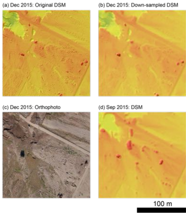
Figure 5: Enlarged views of Fig. 3 images for comparison of the DSMs with different resolutions. (a) Original DSM for December 2015 (resolution: 3.84 cm). (b) Down-sampled DSM for December 2015 (resolution: 1 m). (c) Orthophoto taken in December 2015. (d) DSM for September 2015 (resolution: 1 m). Note that the trivial relief in (a) is largely removed in the down-sampled DSM in (b).
