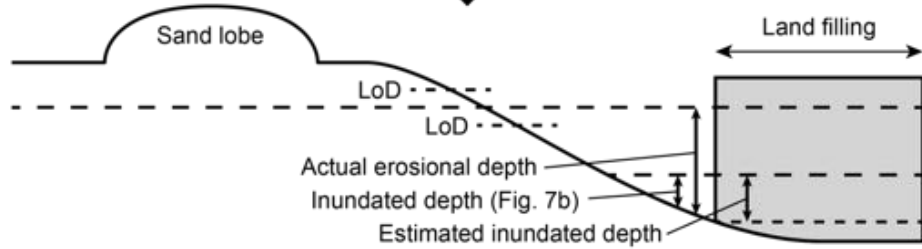
Figure 8: Schematic description of the topographic changes caused by the flood and the later disappearance of inundation water and land filling. Note that elevation changes smaller than the LoD were neglected in the differential rasters and the volume calculations.
