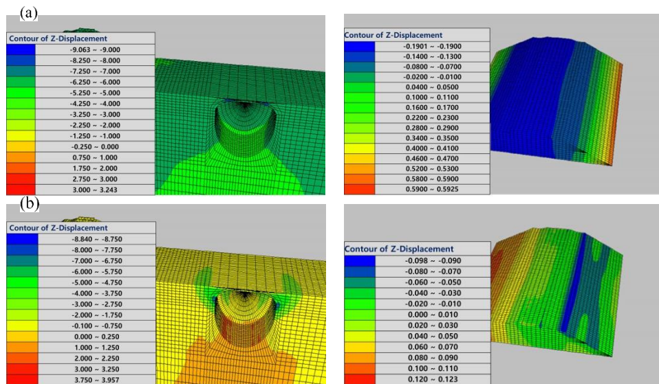
Figure 8. Vertical displacement contours of the roadbed for a cavity diameter 8 m, at the roadbed-to-cavity distance of 25 m: (a) GWL = ground surface and (b) GWL = (-) 8 m.
