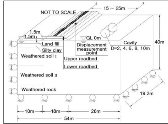
Figure 2. Configuration of the railway roadbed and cavity
