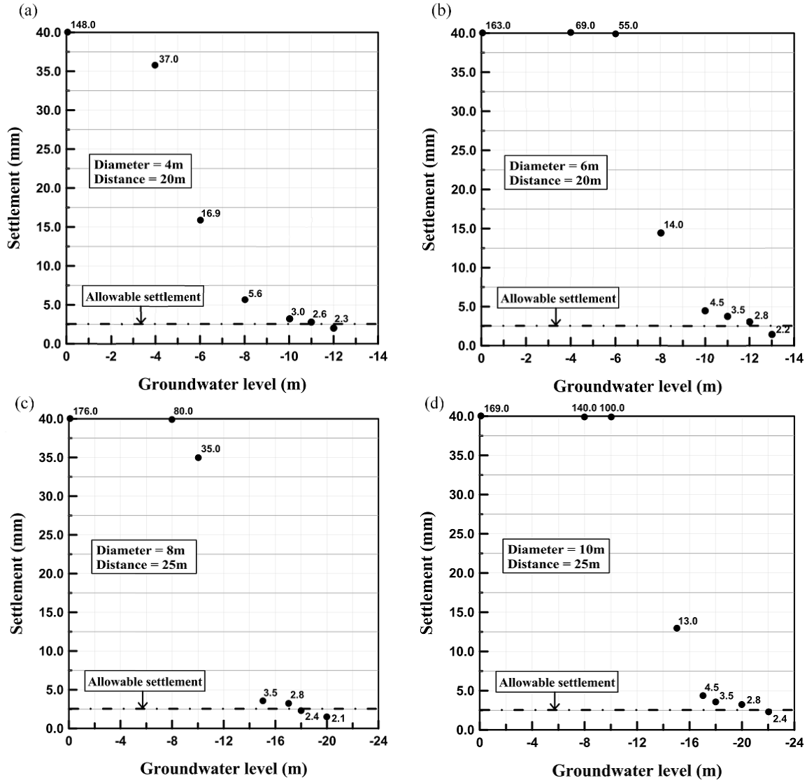
Figure 9. Roadbed settlement with respect to the groundwater level: (a) Diameter of the cavity = 4 m and distance of roadbed from the center of the cavity = 20 m, (b) Diameter of the cavity = 6 m and distance of the roadbed from the center of cavity = 20 m, (c) Diameter of the cavity = 8 m and distance of the roadbed from the center of cavity = 25 m, and (d) Diameter of the cavity = 10 m and the distance of the roadbed from the center of the cavity = 25 m.
