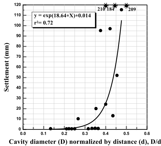
Figure 7. Regression analysis of roadbed settlements with respect to the diameter of the cavity and distance between roadbed and the cavity
