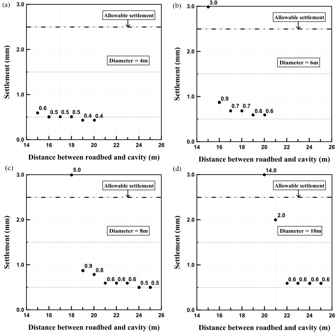
Figure 6. Roadbed settlement with respect to distance between roadbed and cavity: (a) Diameter = 4 m, (b) Diameter = 6 m, (c) Diameter = 8 m, and (d) Diameter = 10 m.
