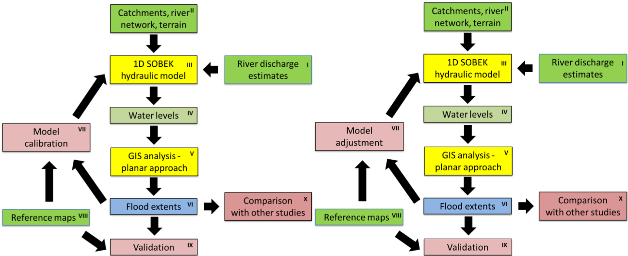
Figure 1. Schematic workflow of flood extents calculation. Roman numerals refer to the text.
