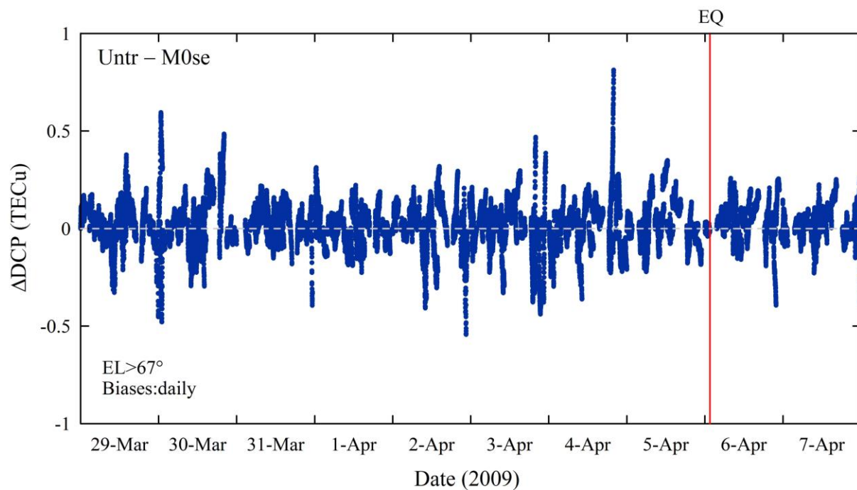
5 Figure 5. Differential carrier phase (DCP) difference \Delta DCP = DCP_{Untr} - DCP_{M0se} between Untr and M0se GPS receivers calculated using the same GPS data of Nenovski et al. (2015) from all satellites crossing central Italy with an elevation angle greater than 67^\circ . The vertical red line identifies the 6 April 2009 main shock.
