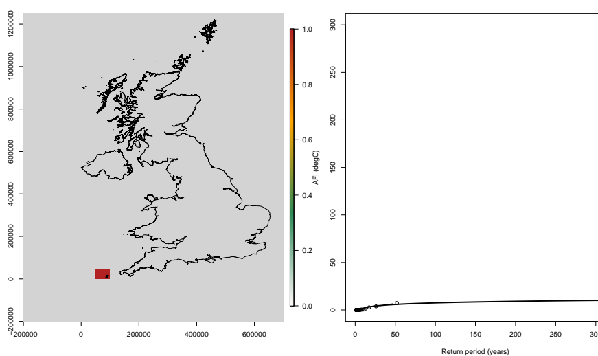
Fig. 1. Weighted AFI RP curve for all cells in UK, based on the historical AFI GEV fit (black circles), the GEV fitted
