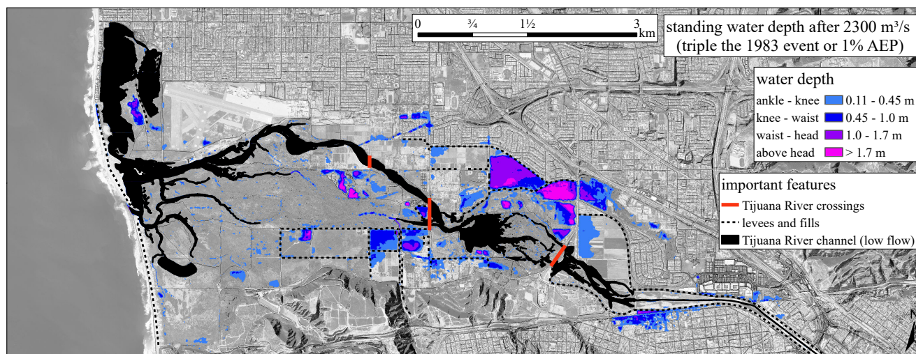
Figure 9. Flood hazard map illustrating pooled water that did not freely drain following a peak Tijuana River flow of 2300 \text{ m}^3/\text{s} , which has an estimated 1% AEP or 100 year frequency. The flood depths shown on the map are the hydraulic model solution after the hydrograph receded to baseflow conditions. The areas that do not freely drain are likely to experience increased mosquito activity and exposure to pollutants following a major flooding event.
