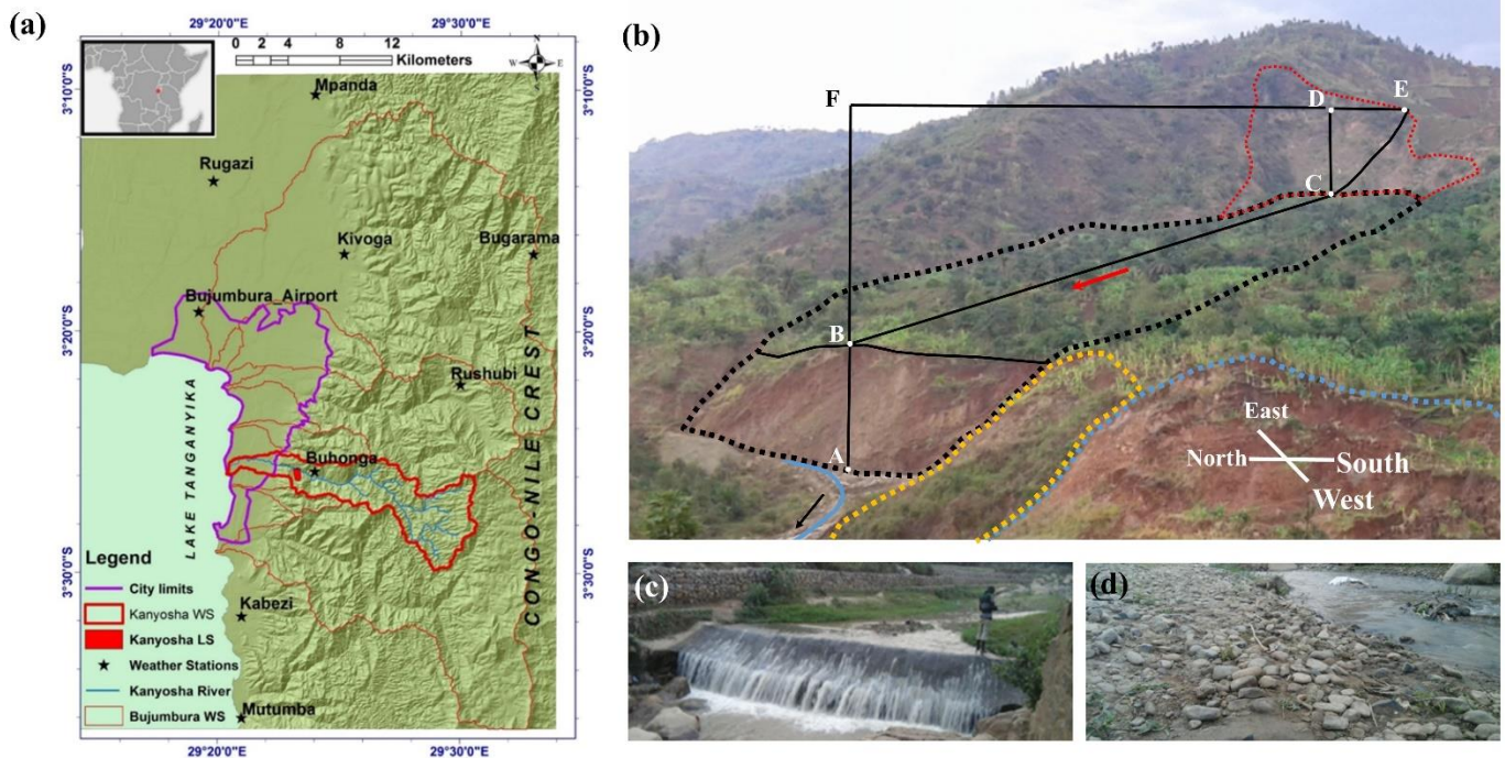
55 Figure 1. (a) Bujumbura region with indication of watersheds of the main rivers, the limits of the city and Lake Tanganyika. The watershed of the Kanyosha River is highlighted in the central part, with the river network inside. The weather stations in and around Bujumbura, the Kanyosha Landslide (in the text called ‘Banana Tree Landslide’, also referred to as BTL, in red contours) and the Congo- Nile crest are also shown. ‘LS’ and ‘WS’ stand for ‘Landslide’ and ‘Watershed’, respectively. (b) View of BTL (black dotted contour) and the main scarp (red 60 dotted contour) as well as its lateral local instabilities (orange and light blue dotted contours). The landslide sliding direction and the river flow direction are indicated by the red and the black arrows, respectively. AB indicates the height (=26 m) of the landslide frontal part near the river; BC outlines the BTL length in the sliding direction (~750 m); CD shows the height of the main scarp (~ 75m) along profile BCE. The blue line indicates the river channel axis. (c) Waterfall over a former flood control structure. (located 270 m downstream of cross-section 3 shown in Fig. 3) (d) View of the river bed during the dry season with presence of cobbles and fine boulders that are deposited after floods during the wet season.
