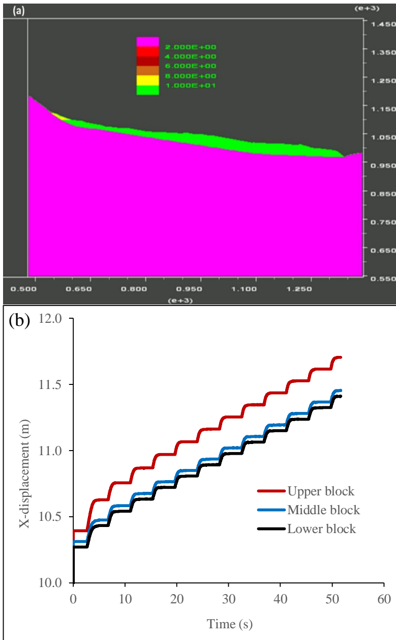
395 Figure 12. Plots of blocks (a) and displacements (b) as given in the UDEC output for run 13 (see Supplement 2, Fig. S1b: using a cohesion of 0.01 MPa and a seismic shaking of 51 seconds).
