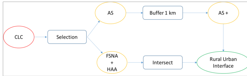
Figure 2 - Framework implemented in the Model Builder (ArcGIS™) to map the rural-urban interface. CLC=CORINE land cover; AS = Artificial surfaces; FSNA = Forest and Semi natural areas; HAA = Heterogeneous Agricultural areas.
