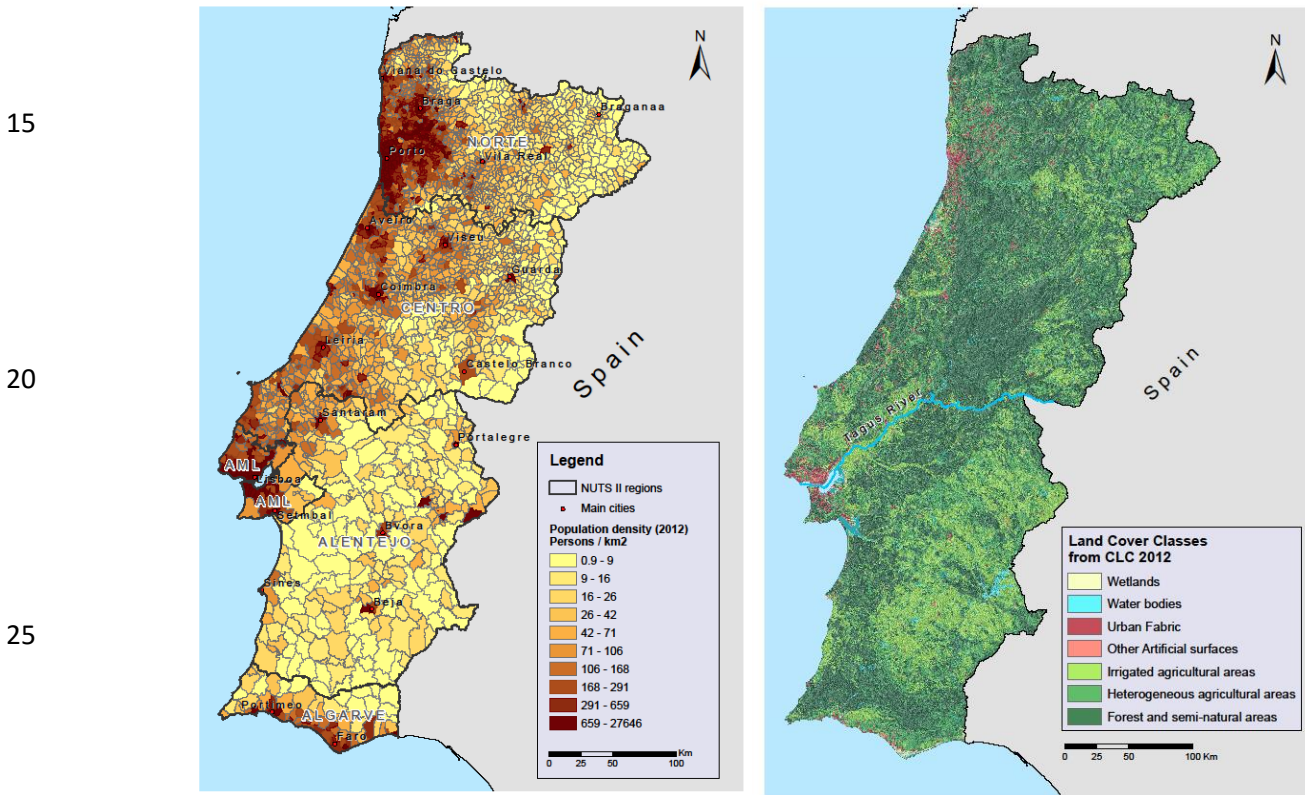
Figure 1 – (Left) Population density at parish level (INE, 2012) in the mainland Portugal, with the location of the of the major cities. NUTS refers to regions according to Nomenclature of Territorial Units for Statistics level II (Eurostat, 2017; Santos, 2014). (Right) Land cover of mainland Portugal based on the second level of CORINE land cover inventory 2012 (EEA, 2016)
