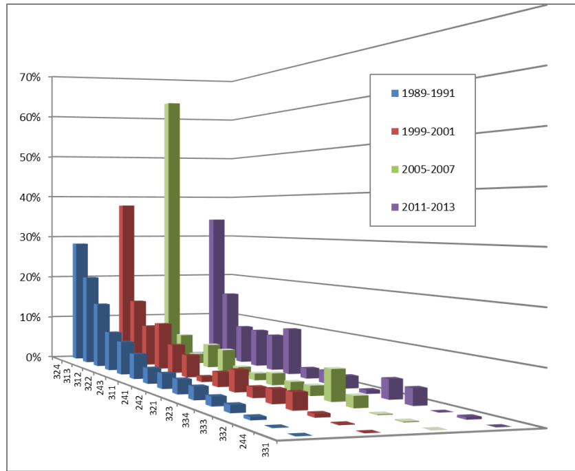
5 Figure 7 – Classes of land use, as defined by the third level hierarchy of CORINE Land Cover, affected by wildfires expressed in percentage as the ratio of burnt area (BA) affecting each CLC classes over the total BA for each frame period.
