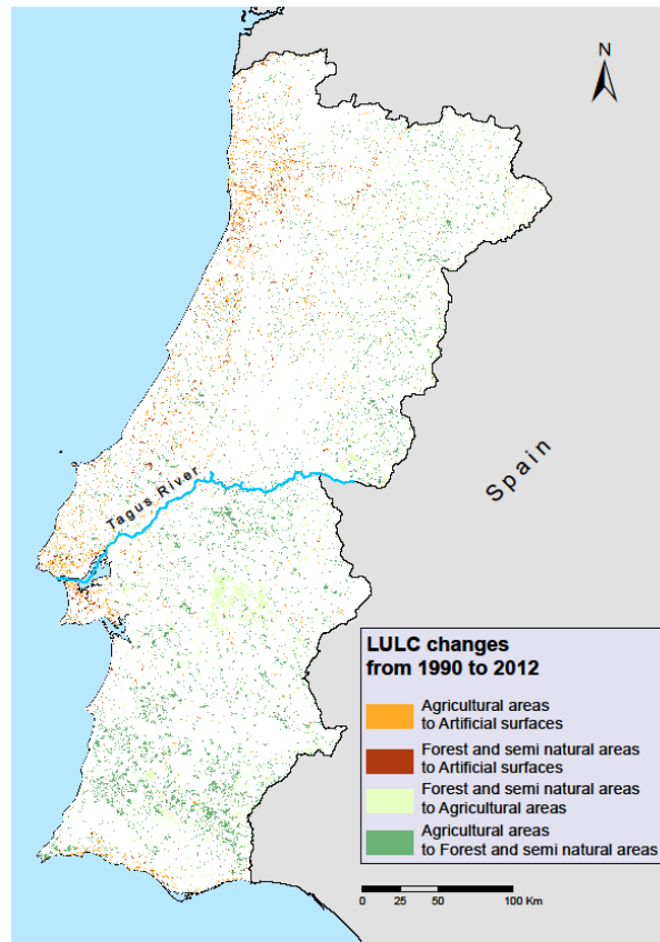
Figure 3 – Map of land cover/land use transition from 1990 and 2012, evaluated considering the first level hierarchy of CLC 1990 and CLC 2012
