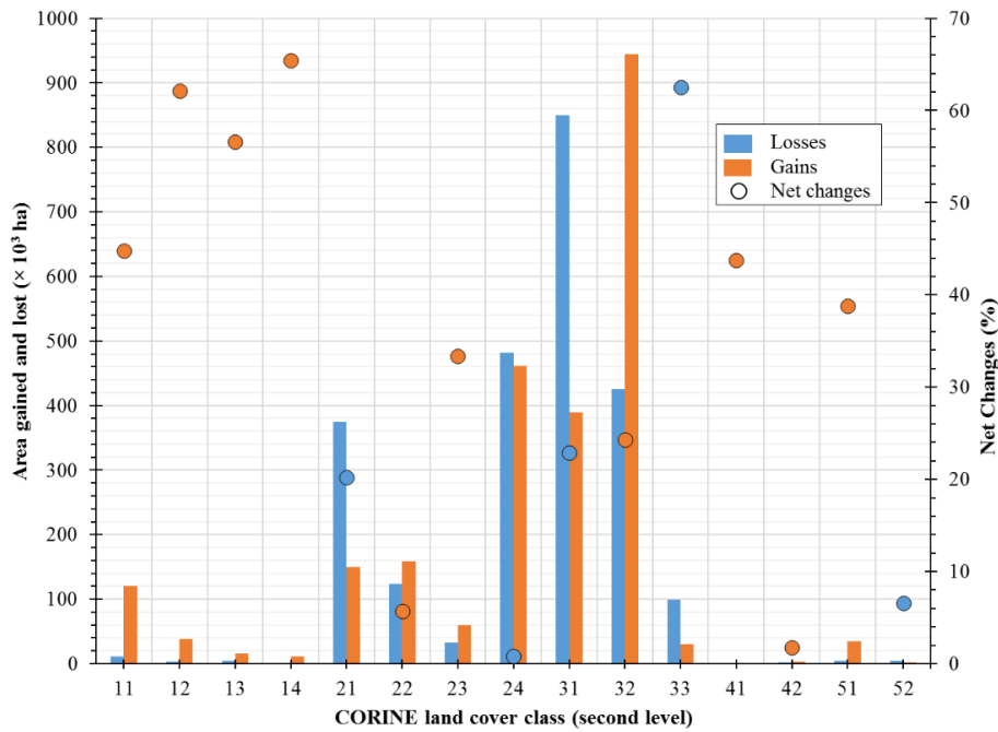
Figure 5 – Area lost and gained from 1990 to 2012 for each CORINE land cover class, considering the second level hierarchy. Net percentage changes were computed relatively to the total area of each class in the later land cover.
