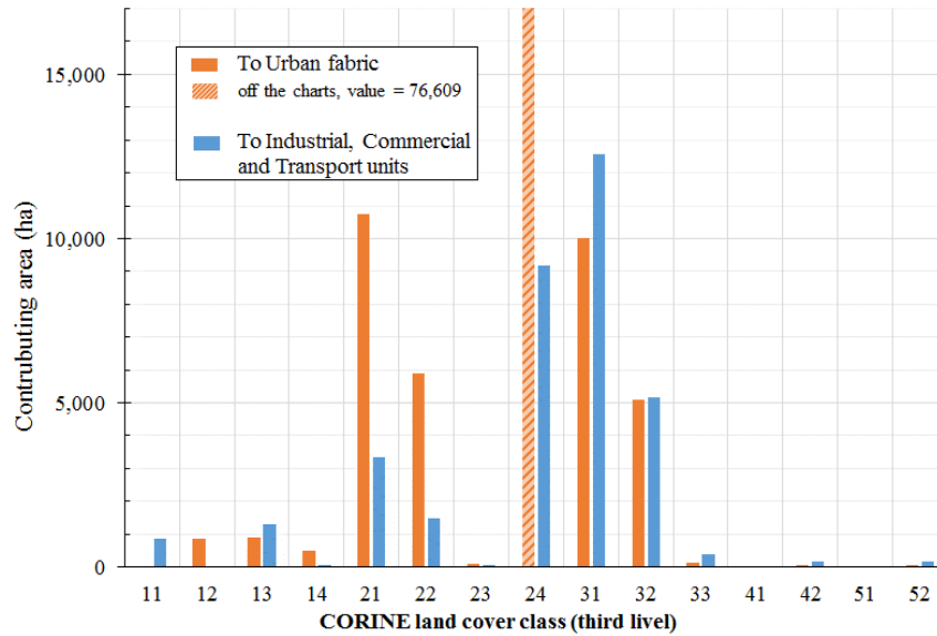
Figure 6 – Contribution to the net changes from 1990 to 2012 of “Urban fabric” (orange bars) and “Industrial, commercial and transport” (blue bars) from the other CLC sub-levels
