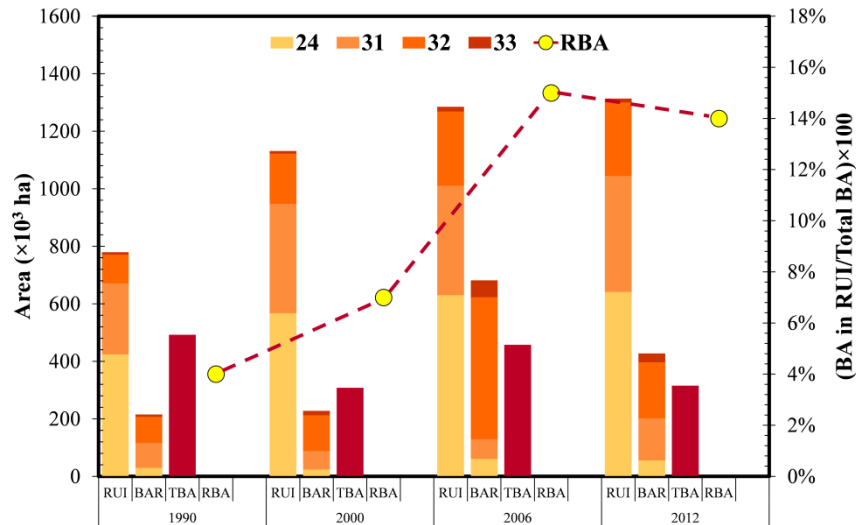
Figure 9 – Evolution of the absolute value of the area of the rural-urban interface (RUI), burnt area within the RUI (RBA), total burnt area (TBA), and relative burnt area within the RUI (RBA, as %), for each investigated period (1990, 2000, 2006, and 2012).
