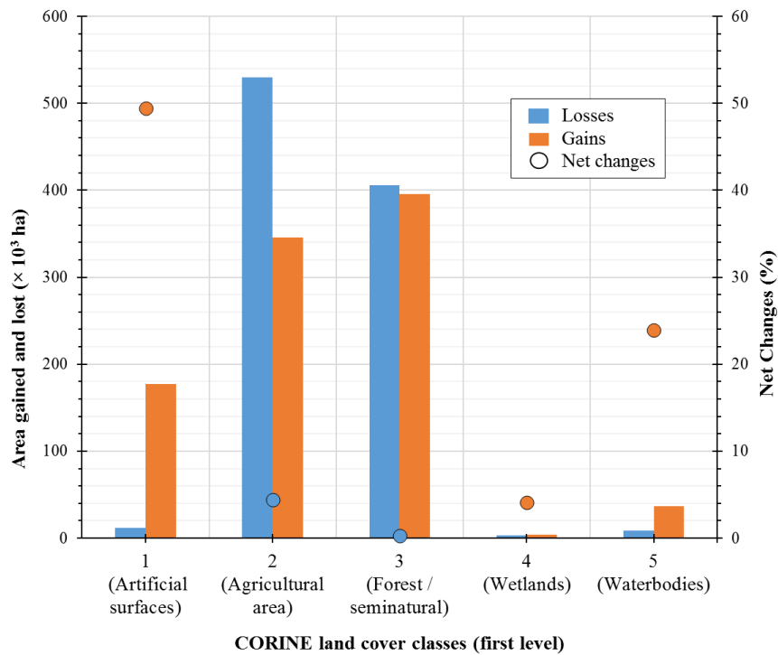
Figure 4 – Area lost and gained from 1990 to 2012 for each CORINE land cover class, considering the first level hierarchy. Net percentage changes were computed relatively to the total area of each class in the later land cover.
