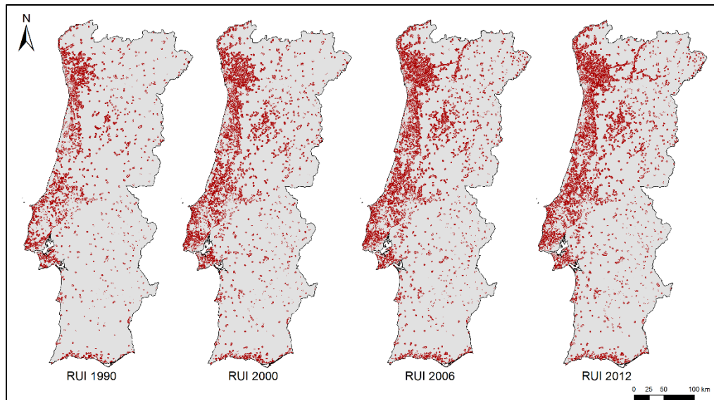
5 Figure 8 – Maps of the rural-urban interface (RUI) in Portugal estimated for the different periods of investigation, and corresponding to the available CORINE Land Cover inventories (1990, 2000, 2006, and 2012)
