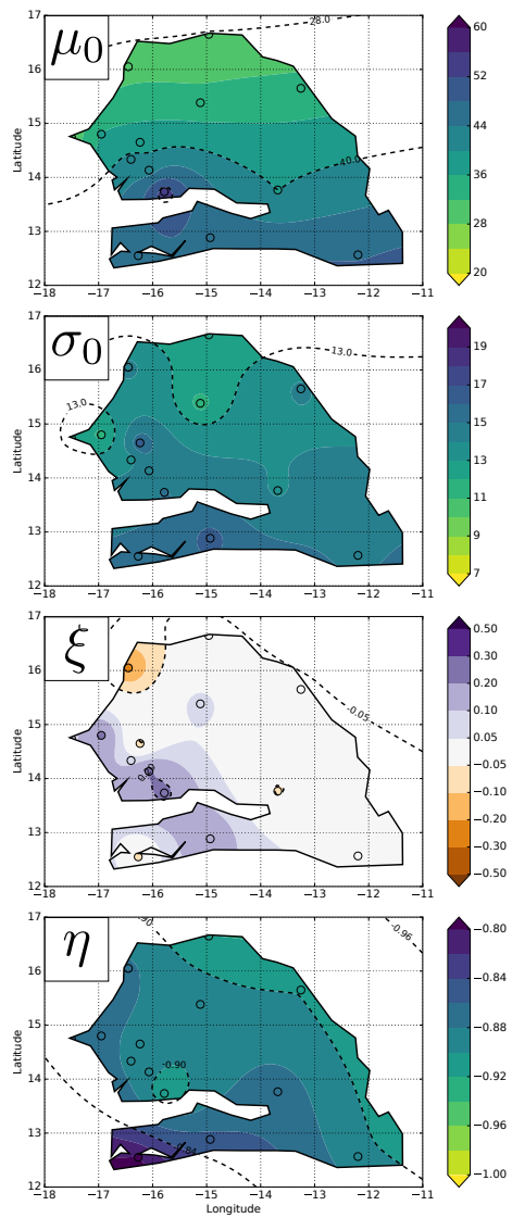
Figure 10. Maps of IDF SiSca parameters: \mu_0 [ \text{mm h}^{-1} ], \sigma_0 [ \text{mm h}^{-1} ], \xi [-], and \eta [-].
