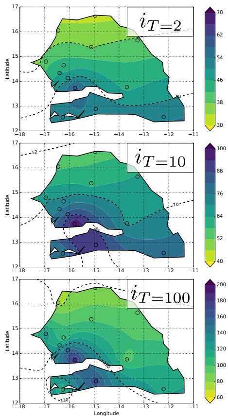
Figure 11. Maps of return levels intensities (from IDF_{SiSca} ) for different return periods ( T=2 , 10, and 100 years from top to bottom) for the reference duration (1h): i_T(D=1) [ \text{mm h}^{-1} ].
