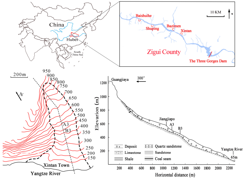
5 Figure 3. Location and plane/section of Xintan Landslide
