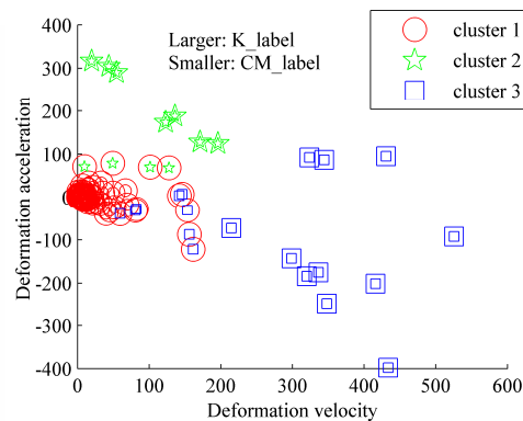
Figure 5. Comparison of K\_label and CM\_label
