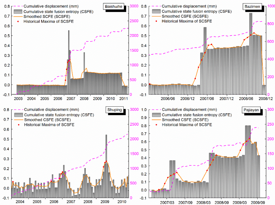
Figure 8. Cumulative state fusion entropy and historical maxima of Baishuihe, Bazimen, Shuping and Pajiayan landslide
