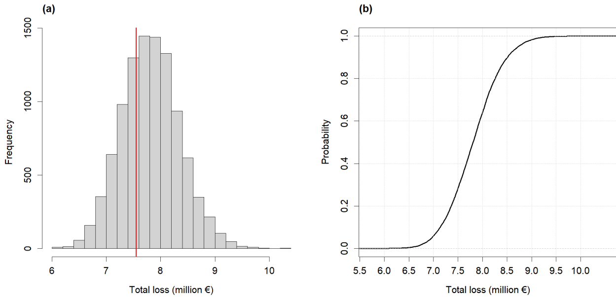
Figure 9: Probabilistic estimates of total loss, relative to model uncertainty, for the Caldagno application case, based on 10 000 realisations of loss to each building. (a) Histogram, with observed loss shown by the vertical red line. (b) Empirical cumulative distribution function (ECDF).
