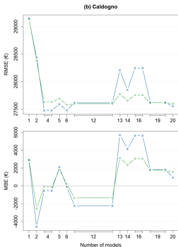
Figure 4: Root mean square error (RMSE) and mean bias error (MBE) of the means of ensembles of increasing size, with models included sequentially from highest to lowest score, starting with the highest ranked single model. Blue crosses and red -green circles refer to ensembles weighted equally and differently, respectively.
