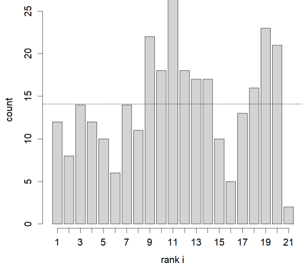
Figure 8: Rank histogram relative to the 20-model ensemble for the Caldogno application case.
