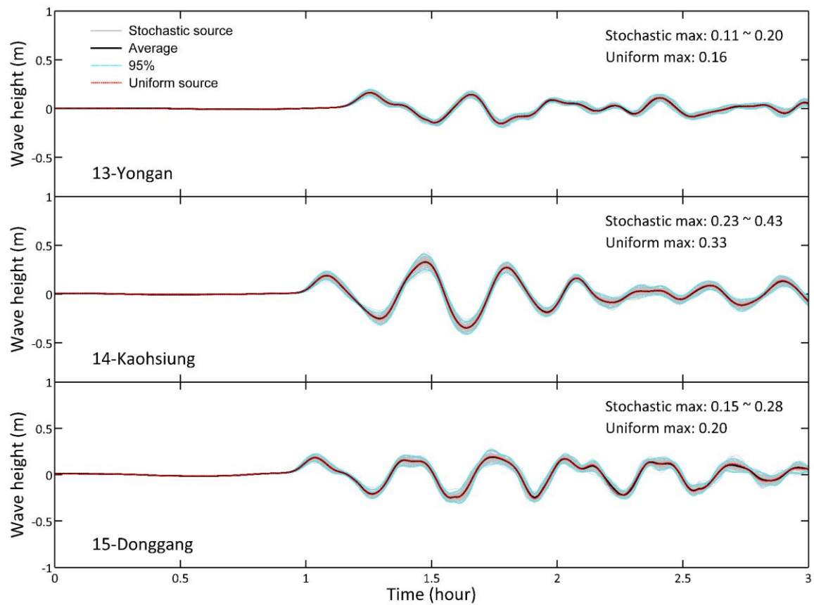
Fig. 5. The time series of wave heights recorded at station 13 (Yongan), 14 (Kaohsiung) and 15 (Donggang).
