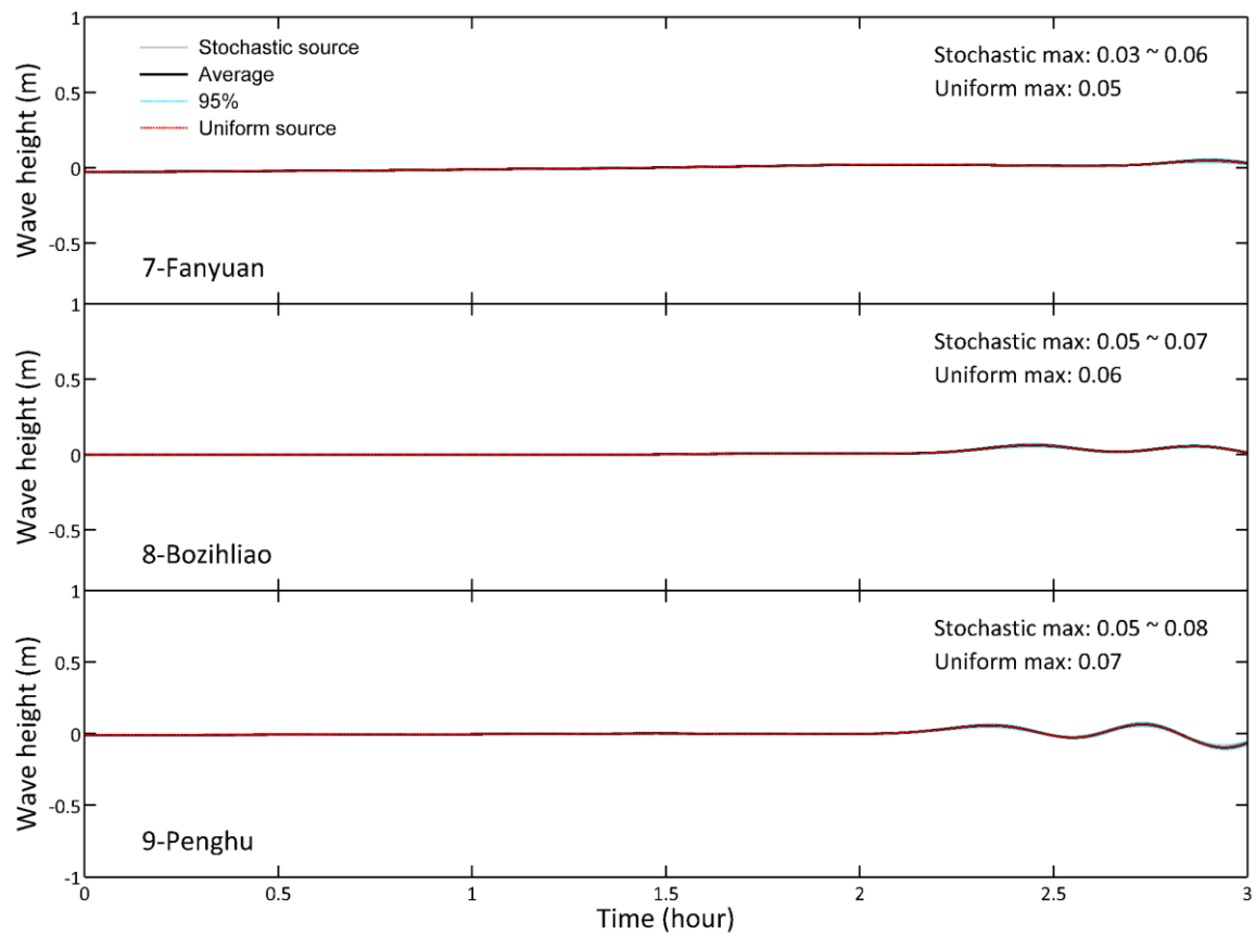
Fig. 3. The time series of wave heights recorded at station 7 (Fanyuan), 8 (Bozihliao) and 9 (Penghu).
