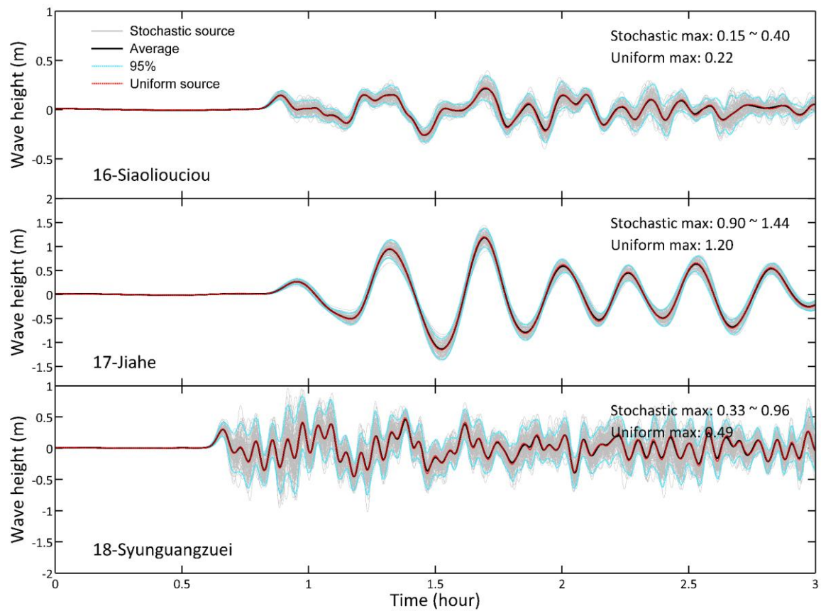
Fig. 6. The time series of wave heights recorded at station 16 (Siaoliouciou), 17 (Jiahe) and 18 (Syunguangzuei).
