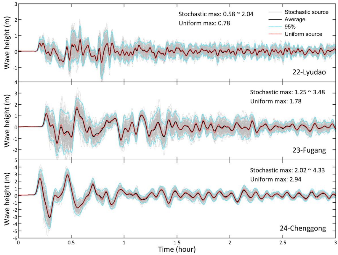
Fig. 8. The time series of wave heights recorded at stations 22 (Lyudao), 23 (Fugang) and 24 (Chenggong).
