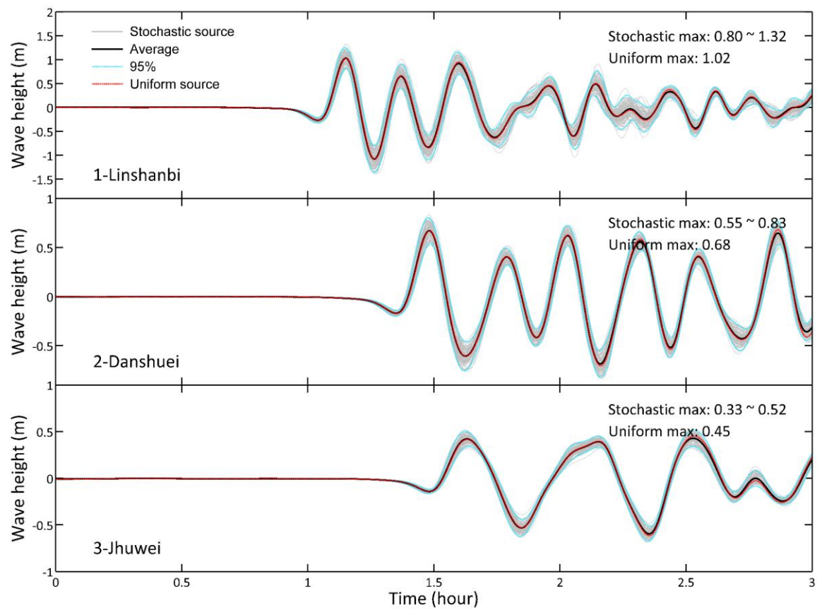
Fig. 1. The time series of wave heights recorded at station 1 (Linshanbi), 2 (Danshuei) and 3 (Jhuwei).
