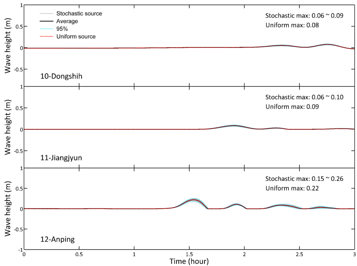
Fig. 4. The time series of wave heights recorded at station 10 (Dongshih), 11 (Jiangjyun) and 12 (Anping).
