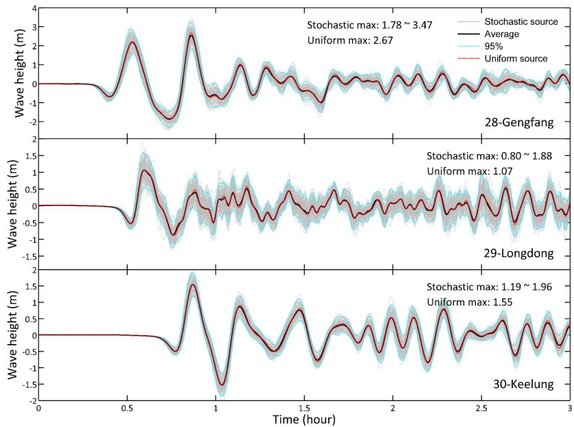
Fig. 9. The time series of wave heights recorded at station 28 (Gengfang), 29 (Longdong) and 30 (Keelung).
