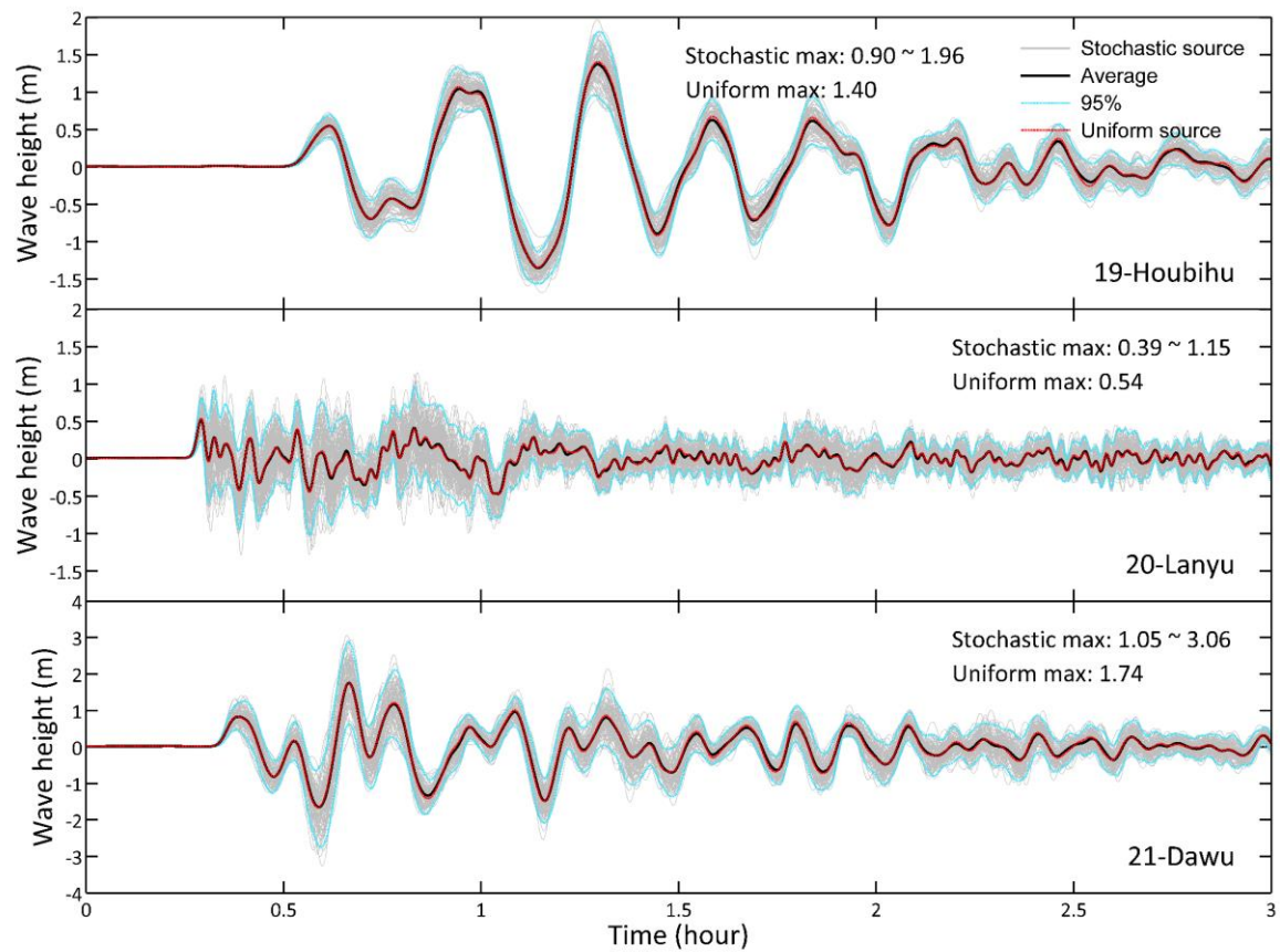
Fig. 7. The time series of wave heights recorded at station 19 (Houbihu), 20 (Lanyu) and 21 (Dawu).
