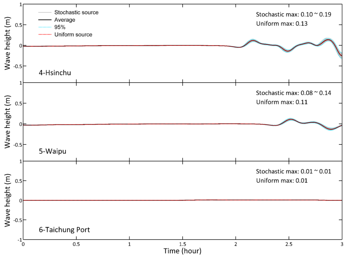
Fig. 2. The time series of wave heights recorded at station 4 (Hsinchu), 5 (Waipu) and 6 (Taichung Port).
