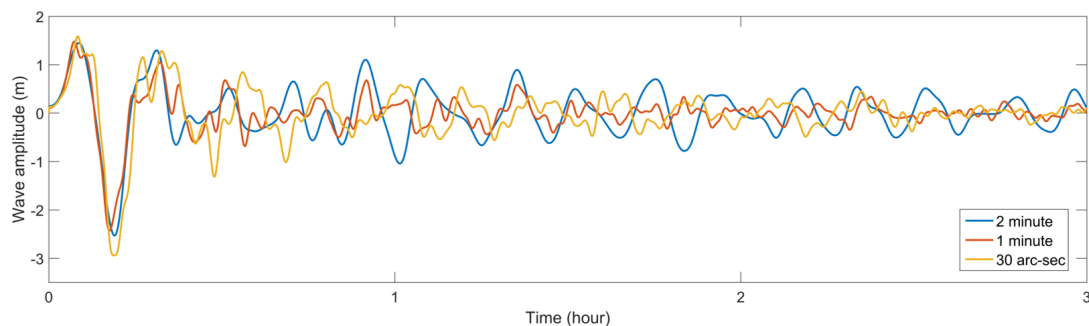
Fig. 1. Fig. 1 The time series by uniform slip distribution at station 25 in different resolution of topography. Blue line is 2 minute, red line is 1 minute and yellow line is 30 arc-sec.
