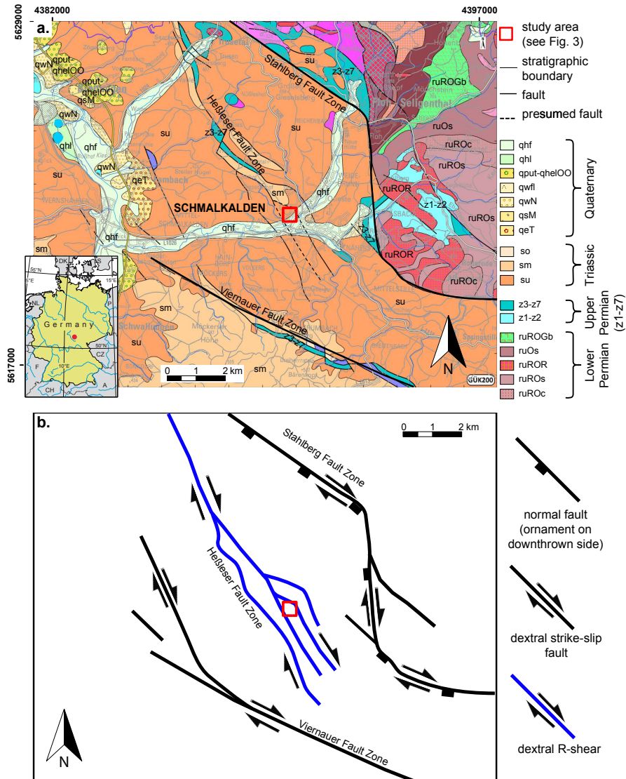
Figure 1. Geological map (a) of Schmalkalden and the surrounding areas (after Bücking, 1906) showing the Heßleser Fault Zone (HFZ) crossing the position of the sinkhole (red square). In the lower left corner a map of Germany with the position of Schmalkalden is shown (red dot). The Mesozoic movements reactivated the tectonic faults (b) and lead to the formation of a dextral strike-slip fault zone which includes the Stahlberg Fault Zone (SFZ) and the Viernauer Fault Zone (VFZ). The HFZ connects the two major faults at an acute angle of 30°. We interpret this as a Riedel R-shear also dextral in movement (see text). For an explanation of the stratigraphic abbreviations, see LBEG (2015).
