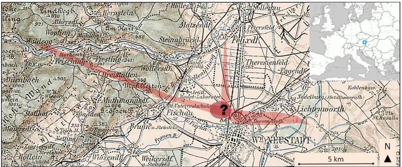
Fig. 2: Map of tornado damage tracks (red shadings) in the Wiener Neustadt area. The hatched area with the question mark denotes the airfield west of town, where the exact genesis of the main tornado is unknown. Basis map: „Generalkarte von Mitteleuropa des k.u.k. Militärgeographischen Instituts Wien, Blatt 34° 48° Wien“ of 1893.
