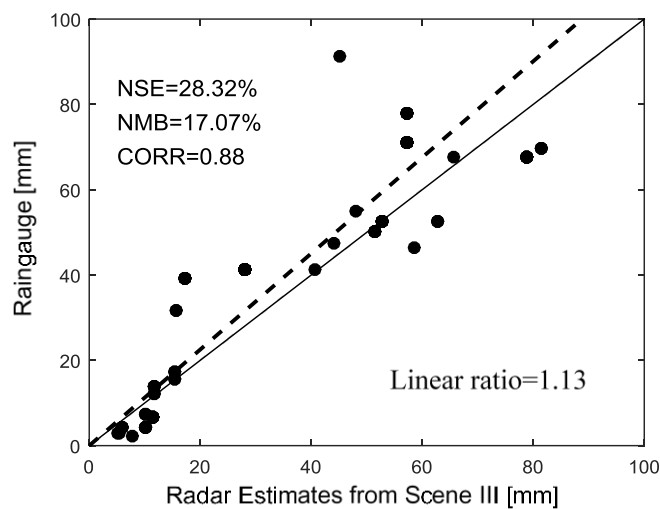
Figure 9. Event-rainfall scatter plots of rain gauges closest to debris flow locations and radar-based estimate from scene III over the same location of rain gauge.
