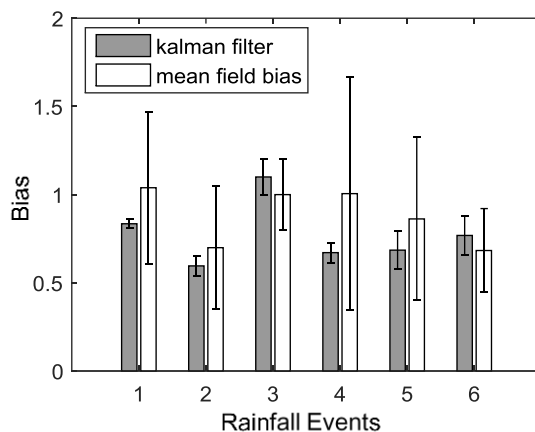
Figure 7. The average and covariance of bias estimation by Kalman filter and mean field bias method for six rainfall event.
