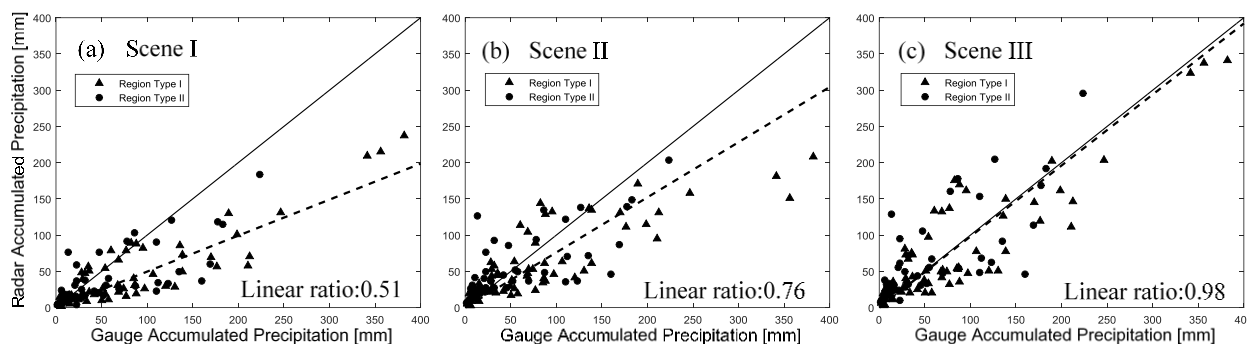
Figure 6. Scatter plots of radar and rain gauge event-rainfall accumulations. (a) Scene1: radar estimate from hybrid scan. (b) Scene 2: radar estimate from hybrid scan and VPR. (c) Scene 3: radar estimate through the hybrid scan, VPR and bias correction.
