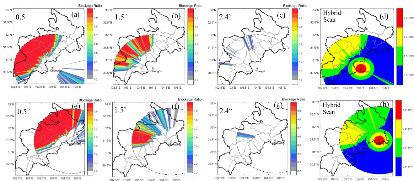
Figure 3. Blockage ratio of beam shielding for the radar main lobe beam and hybrid scan map. (a)-(c) represent the blockage ratio of Chengdu radar at the elevations of 0.5°, 1.5° and 2.4° respectively. (e)-(f) represent the blockage ratio of Mianyang radar at the elevations of 0.5°, 1.5° and 2.4° respectively. Hybrid scan maps for Chengdu and Mianyang are merged under the condition of blockage ratio is lower than 0.5.
