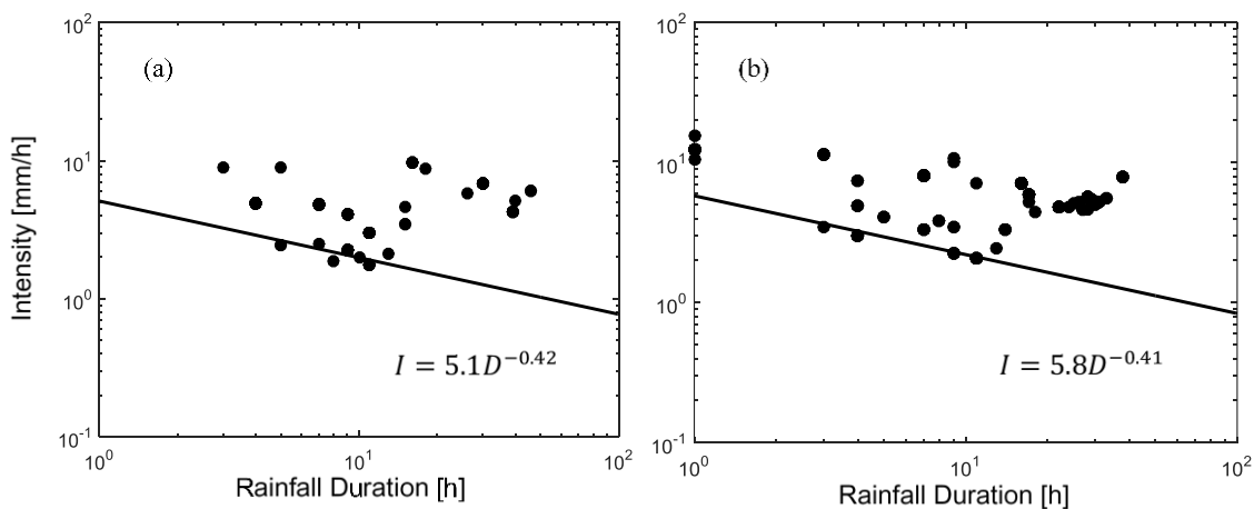
Figure 10. Intensity–duration thresholds (black line) derived from (a) rain gauges closest to debris flow locations and (b) radar rainfall estimation at the same location of the rain gauges closest to the debris flow.
