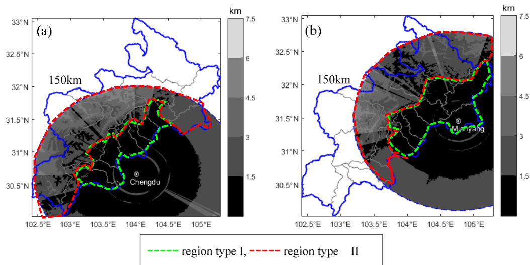
Figure 5. The height from the ground of hybrid scan for two S-band radar (a) radar located at Chengdu (b) radar located at Mianyang. The regions surrounded by green dash lines meet the condition of that the height from the ground is 1.5 km below and the distance from radar is inner 100 km and is recognized as region type I. The regions surrounded by the red dash lines represents the area under the opposite condition and is recognized as region type II.
