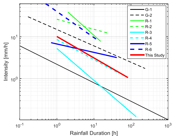
5 Figure 11. I–D thresholds determined for this study (red line) and those of various other studies. G = global, R = region. G-1: Guzzetti et al. (2008); G-2: Caine (1980); R-1: Wenchuan earthquake area, Wei and Tang(2014); R-2: Qingping, a region in Wenchuan earthquake area, Tang et al. (2012); R-3: Wenchuan earthquake area, Xiaojun G. et al.(2016); R-4:Italy, Francesco M. et al.(2014); R-5 Central Taiwan, Jan and Chen(2005);R-6 Japan, Jibson (1989).
