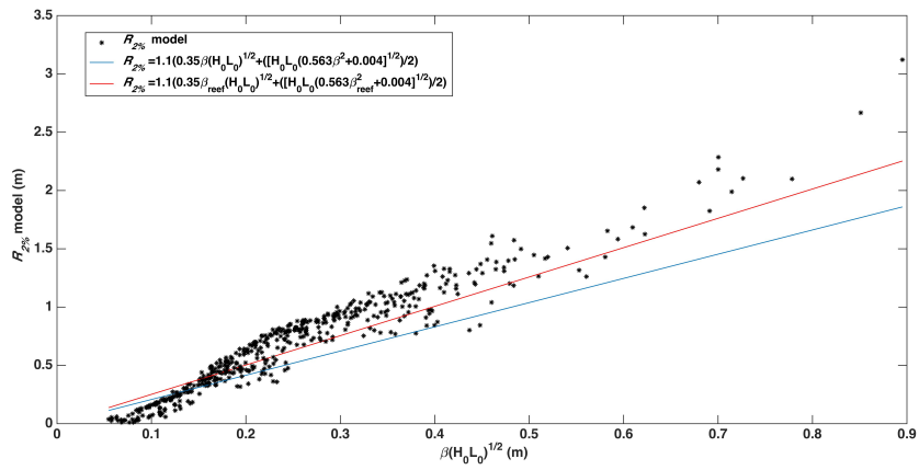
Figure 10. Extreme runup values ( R_{2\%} ) for the selected 30-year hindcast data (black dots) and the complete parameterisation suggested by Stockdon et al. (2006) with the beach face slope (blue line) and reef face slope (red line).
