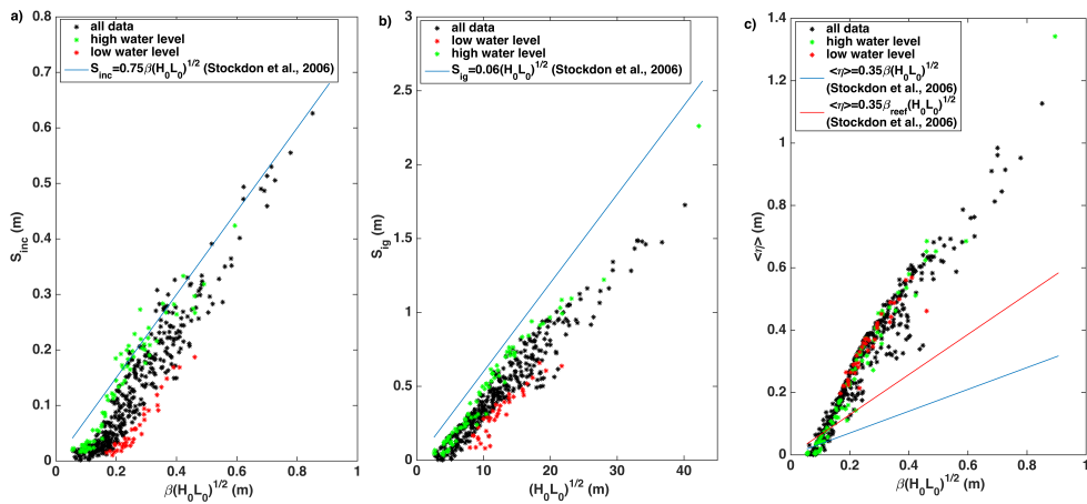
Figure 9. (a) Incident swash, (b) infragravity swash and (c) wave setup parameterised in a dimensional form of the Iribarren equation and in comparison to Stockdon et al. (2006) (blue lines) and a modified form for wave setup, which includes the reef face slope (red line). Black dots represent the selected hindcast cases, green the values associated with high water levels ( Z \geq Z_{15\%} = 0.1636 m) and red those associated with low water levels ( Z \leq Z_{15\%} = -0.1636 m).
