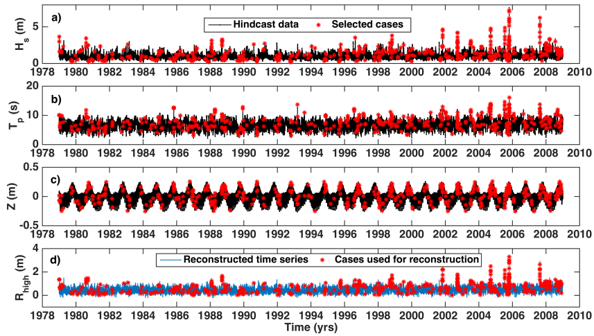
5 | Figure 2. Reconstructed time series, including the extreme water level, R_{high} , for the current reef profile using the 30-year hindcast wave conditions (wave height and period; H_s and T_p ) and sea level (astronomical tide without storm surge) ( Z ). (a)–(c) Black lines indicate available hindcast data and red stars indicate the selected cases used to represent the complete time series. (d) Blue line represents time series reconstructed from the simulated results. Red stars indicate the cases used for reconstruction. R_{high} = R_{2\%} + Z .
