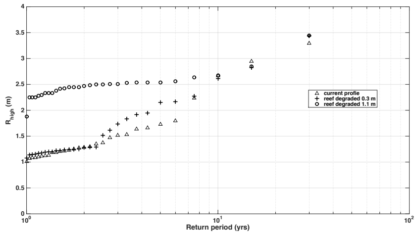
Figure 5. Return value of R_{high} for the current reef profile (triangles), the reef degraded by 0.3 m (crosses) and for the profile with the reef degraded by 1.1 m (open circles).
