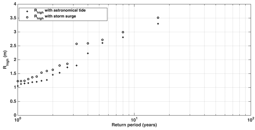
Figure 7. Return value of R_{high} for the model run with the storm surge (open circles) and without (crosses) for the time period of 1993-2008.
