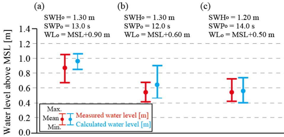
5 Figure 2: Comparison of in situ measurements and calculated results of water levels on the reef flat (400 m from the shore) at the study site. (a) Test1: The assumed SWH_o and SWP_o values were 1.30 m and 13.0 s, respectively. The assumed WL_o value was +0.90 m above MSL. (b) Test 2: The assumed SWH_o and SWP_o values were 1.30 m and 12.0 s, respectively. The assumed WL_o value was +0.60 m above MSL. (c) Test 3: The assumed SWH_o and SWP_o values were 1.20 m and 13.0 s, respectively. The assumed WL_o value was +0.50 m above MSL.
