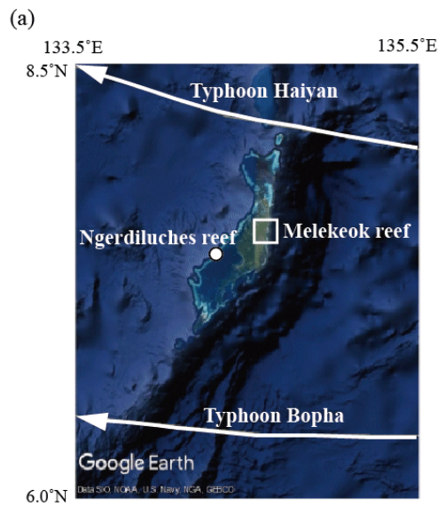
Figure 1: Location of Melekeok reef in the Palau Islands, and the reef topography used for wave calculations. (a) Location of Melekeok reef. The open circle indicates the drillcore site on Ngerdiluches reef (Kayanne et al., 2002). Typhoon Bopha passed south of Palau Islands on 2 December 2012 and Typhoon Haiyan passed north of the islands on 6–7 November 2013, provided by Digital Typhoon ( http://agora.ex.nii.ac.jp/digital-typhoon/index.html.en ).
