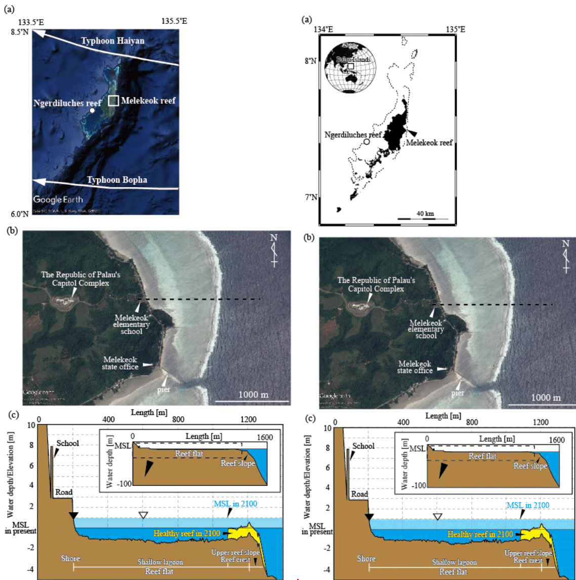
Figure 14: Location of Melekeok reef in the Palau Islands, and the reef topography used for wave calculations. (a) Location of Melekeok reef. The open circle indicates the drillcore site on Ngerdiluches reef (Kayanne et al., 2002). Typhoon Bopha passed south of Palau Islands on 2 December 2012 and Typhoon Haiyan passed north of the islands on 6–7 November 2013, provided by Digital Typhoon ( http://agora.ex.nii.ac.jp/digital-typhoon/index.html.en ). (b) Satellite image of the reefs, long beaches, the Republic of Palau's Capitol Complex, Melekeok elementary school, and Melekeok state office. The dashed line shows the location of the survey transect. (c) The measured cross-section, showing the present day and the 2100 reef topography. The reef crest and upper reef slope will be characterized by upward reef growth or cessation of growth in response to sea level rise (SLR). This figure shows the example of upward reef growth for a healthy reef in response to +0.98 m SLR in 2100, based on the Representative Concentration Pathway (RCP) 8.5 scenario (Church et al.,
