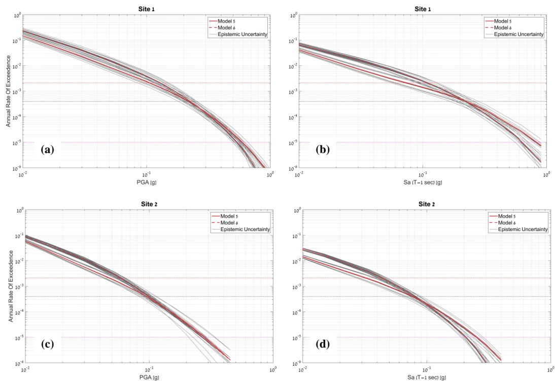
Figure 10. Hazard curves for Models 5 and 6, showing the full range of parametric uncertainty, for (a) Site #1 at T=0.01\text{sec} , (b) Site #1 at T=1.0\text{sec} , (c) Site #2 at T=0.01\text{sec} , and (d) Site #2 at T=1.0\text{sec} .
