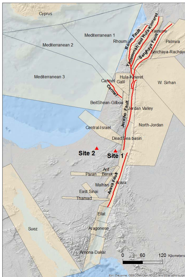
Figure 2. The seismotectonic model proposed by Davis and Dor (2014), combining linear faults with buffer zones and areal source zones for seismic sources with no defined underlying faults.
