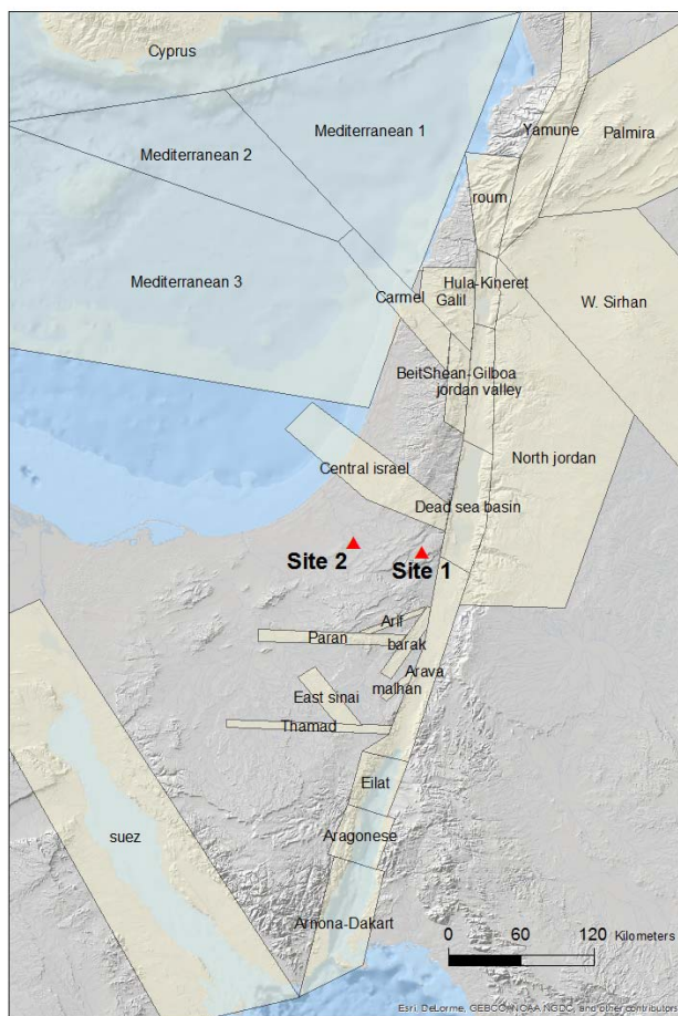
5 Figure 1. The seismotectonic model underlying the SI413 map (Klar 2011). All seismic sources are represented as areal source zones.
