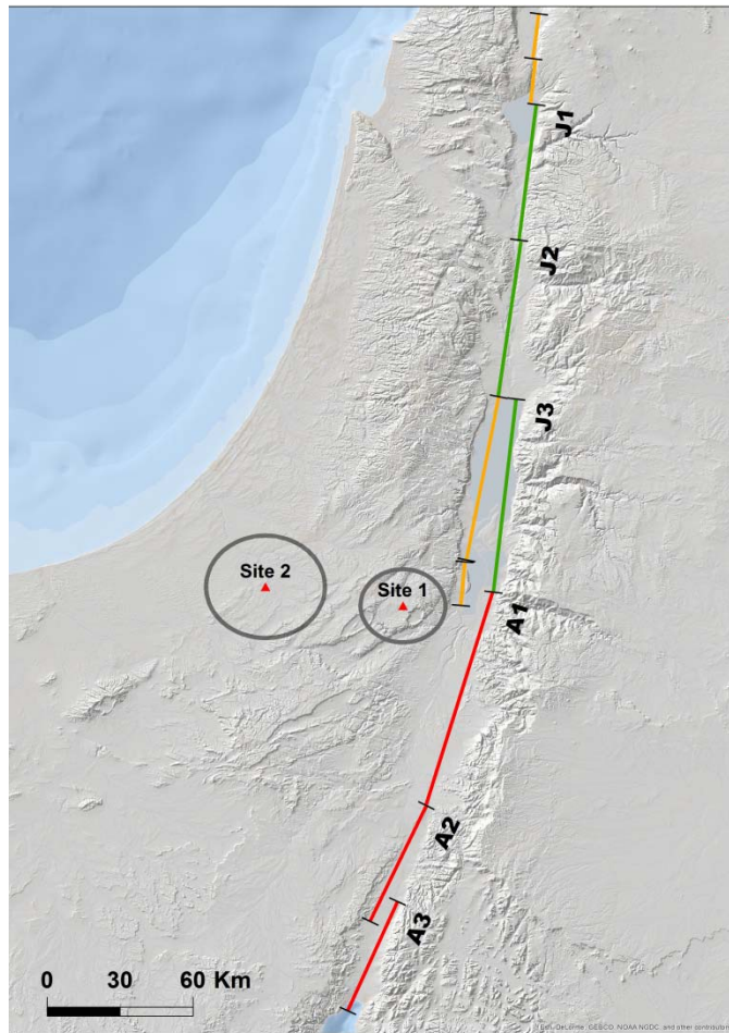
Figure 6. The segmented model of the DST, in which the Arava and Jericho faults are each represented by three segments. The Arava fault is represented by the red lines numbered A1 through A3. The Jericho fault is represented by the green lines numbered J1 through J3. Orange lines represent segments which were not included in the analysis herein, to avoid double-counting of moment release.
