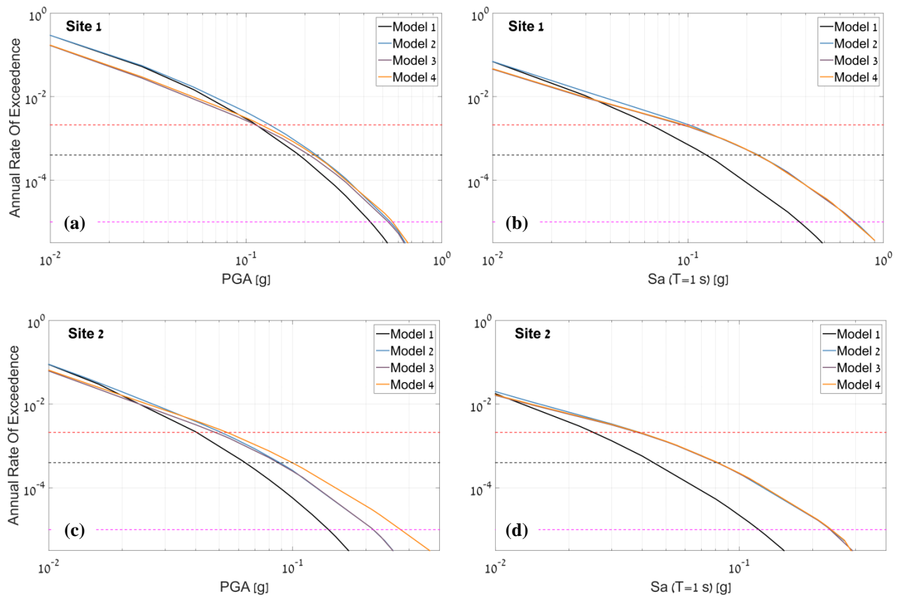
5 Figure 9. Hazard curves obtained using Models 1 through 4 for (a) Site #1 at T=0.01s , (b) Site #1 at T=1.0s , (c) Site #2 at T=0.01s , and (d) Site #2 at T=1.0s .
