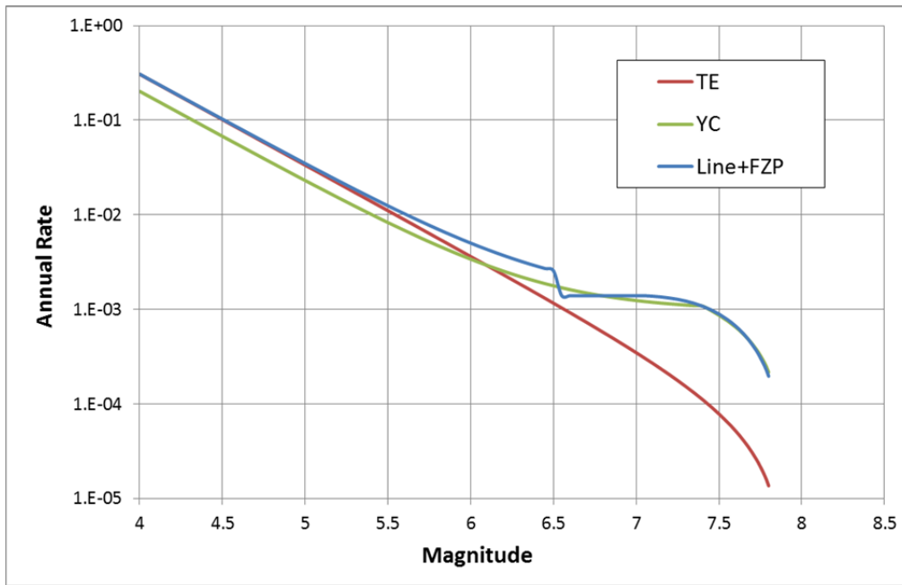
Figure 3. Magnitude-frequency distributions for the 191-km continuous Arava Fault segment. TE – equivalent to Model 1, with the associated activity rate of N(M_{\min}=4.0) = 0.3 , which is equivalent to a slip-rate of 0.6 mm/year. Line+FZP – equivalent to Model 2, in which the FZP has the same parameters as in Model 1 and the linear fault source has the same parameters as in Model 3. YC – equivalent to Model 3, in which the fault is assigned a composite model with a slip-rate of 3.5 mm/yr.
