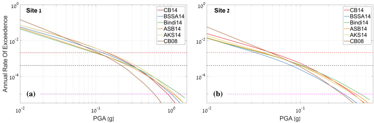
Figure 12. Hazard curves for Model 5, using the average weighted values, at (a) Site #1, and (b) Site #2.
