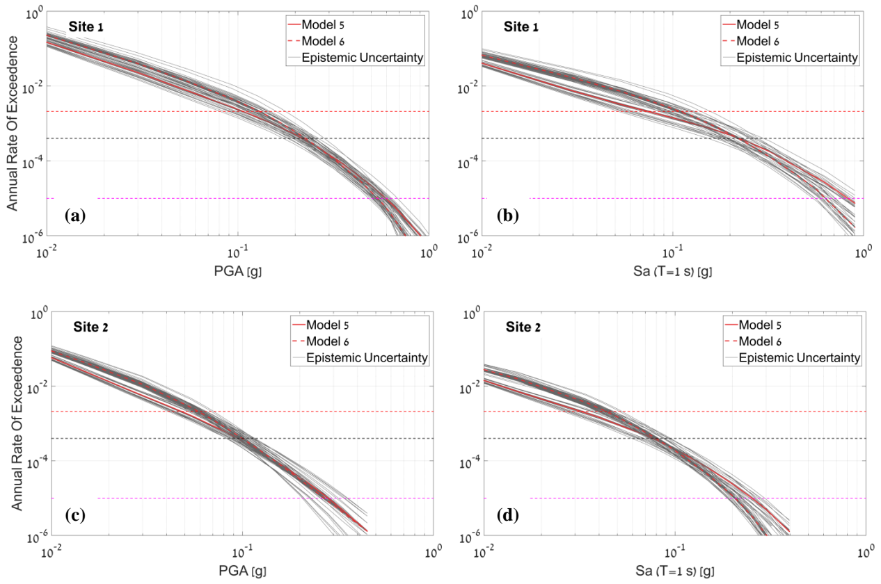
Figure 10. Hazard curves for Models 5 and 6, showing the full range of parametric uncertainty, for (a) Site #1 at T=0.01s , (b) Site #1 at T=1.0s , (c) Site #2 at T=0.01s , and (d) Site #2 at T=1.0s . The weighted averages are represented by the red curves.
