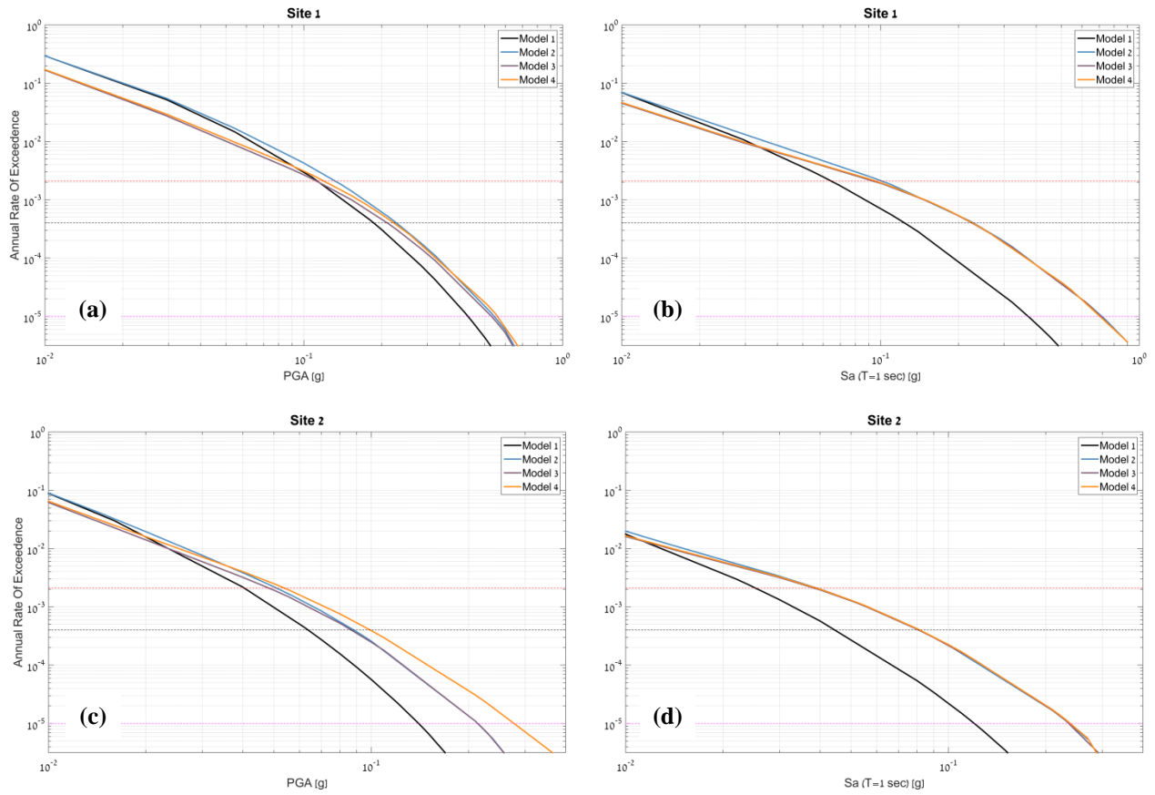
5 Figure 9. Hazard curves obtained using Models 1 through 4 for (a) Site #1 at T=0.01sec, (b) Site #1 at T=1.0sec, (c) Site #2 at T=0.01sec, and (d) Site #2 at T=1.0sec.
