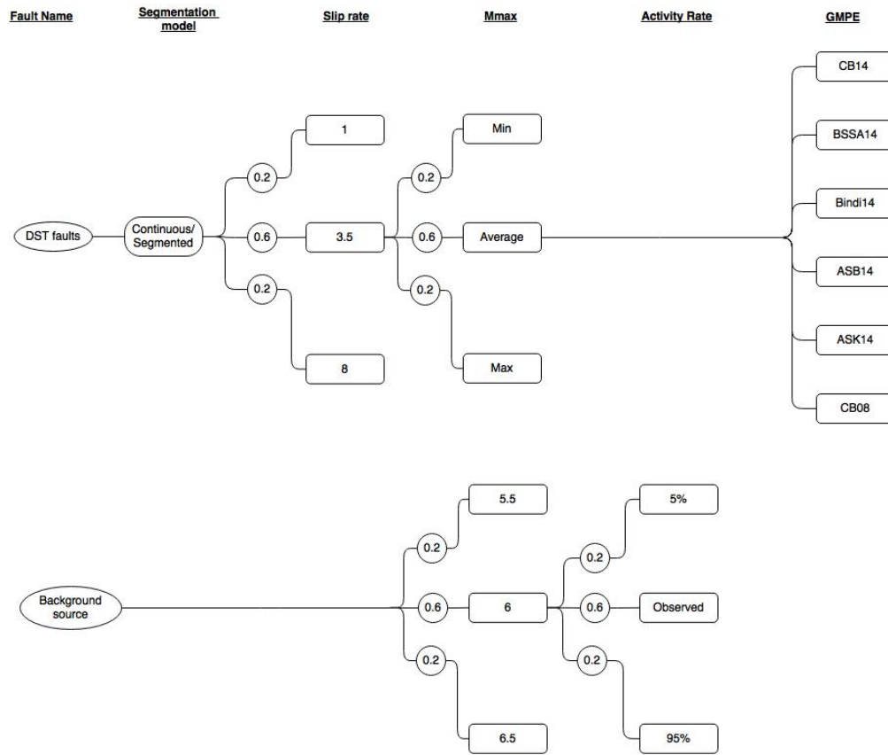
Figure 8. Logic tree for Model 5, showing the main branches of the linear sources (top) and the background polygon (bottom). Where a weight isn't assigned, the analysis was conducted separately for each alternative.
