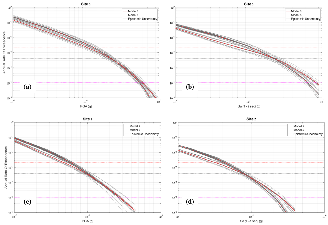
Figure 10. Hazard curves for Models 5 and 6, showing the full range of parametric uncertainty, for (a) Site #1 at T=0.01 sec, (b) Site #1 at T=1.0 sec, (c) Site #2 at T=0.01 sec, and (d) Site #2 at T=1.0 sec. The weighted averages are represented by the red curves.
