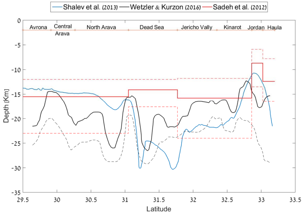
5 Figure 7. The range of evaluations for the seismogenic crustal depth along the DST, based on three independent studies. The X-axis represents a cross section along the DST – from South (left) to North (right). The figure is drawn at a vertical exaggeration of 11. In the Wetzler and Kurzon (2016) study – the solid line represents the 75 th percentile while the dashed line represent the 95 th percentile. In the Sadeh et al. (2012) study – the solid line represents the estimated depth with a confidence level of 68%, while the dashed lines represent two standard-deviations above and below that estimate.
