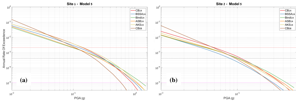
Figure 12. Hazard curves for Model 5, using the average weighted values, at (a) Site #1, and (b) Site #2.
