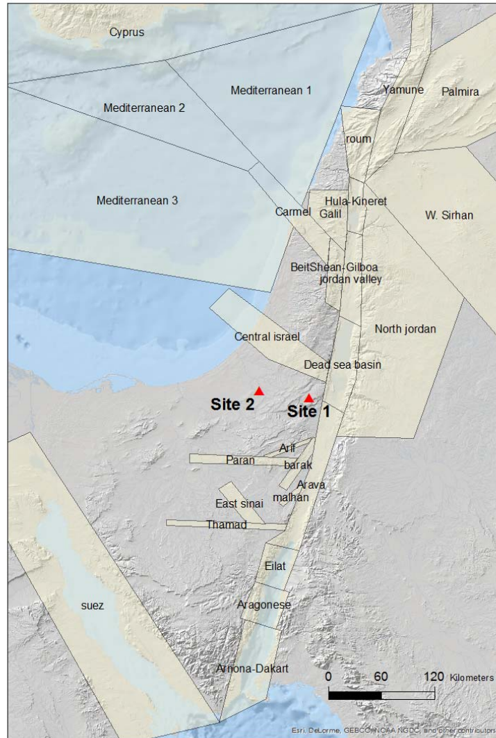
5 Figure 1. The seismotectonic model underlying the SI413 map (Klar 2011). All seismic sources are represented as areal source zones. The boundary coordinates and seismicity parameters associated with this model are available as supplementary material in the electronic appendix.
