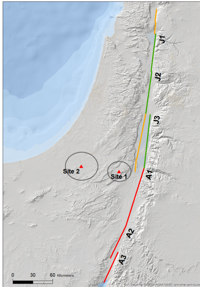
Figure 6. The segmented model of the DST, in which the Arava and Jericho are each represented by three segments. Arava is represented by the red faults numbered A1 through A3. Jericho is represented by the green faults numbered J1 through J3. Orange segments were not included in the analysis herein, to avoid double-counting of moment release.
