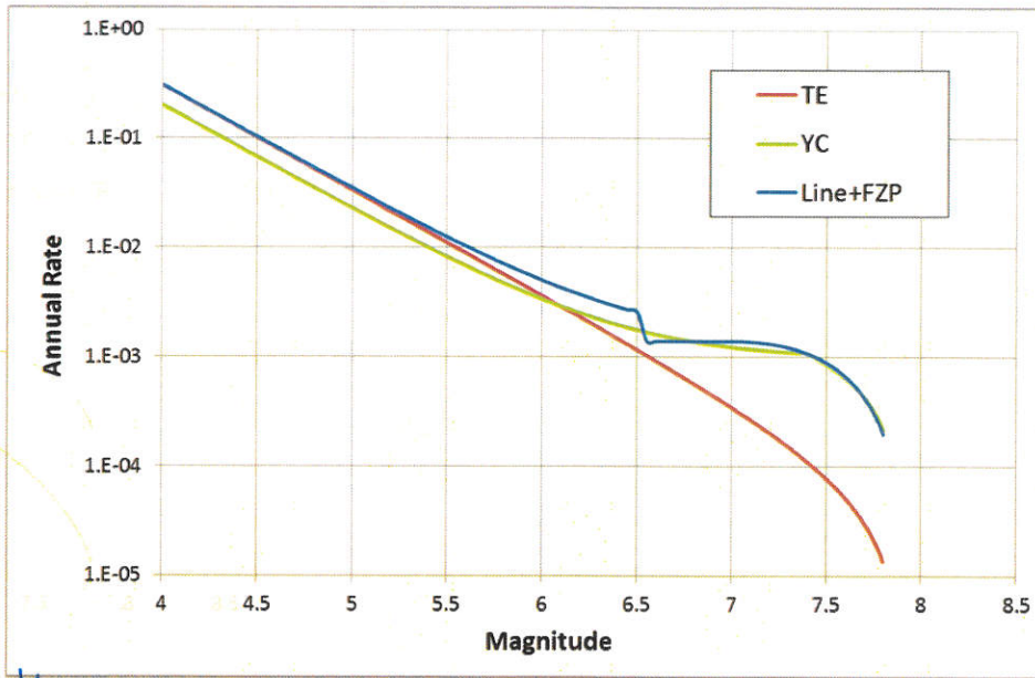
Figure 3. Example magnitude-frequency distributions for the 191-km continuous Arava Fault segment. TE – equivalent to Model 1, with the associated activity rate of N(M_{\min}=4.0) = 0.3 , which is equivalent to a slip-rate of 0.6 mm/year. Line+FZP – equivalent to Model 2, in which the FZP has the same parameters as in Model 1 and the line has the same parameters as in Model 3. YC – equivalent to Model 3, in which the fault is assigned a composite model with a slip-rate of 3.5 mm/year.
