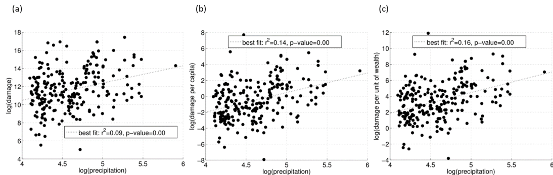
Fig. 2. Scatter plot between basin-aggregated maximum precipitation in 24 h and (a) total damages (D); (b) damage per capita (DPC); and (c) damage per unit of wealth (DPW), for flood events recorded in Catalo
