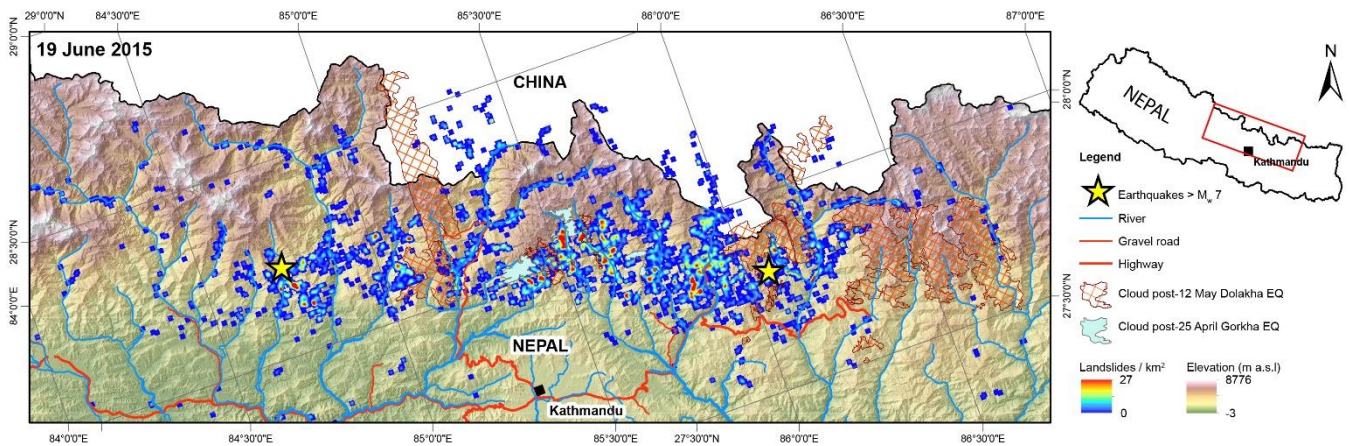
5 Figure 6: Extract from map released on 19 June 2015 containing landslide data from both earthquakes, comprising ~4 500 triggered by the Gorkha event, ~300 by the Dolakha event, and ~800 that could be attributed to either. Orange hatched pattern highlights areas that could not be mapped following the Dolakha earthquake event. Turquoise pattern (direct north of Kathmandu) highlight areas that remained unmapped following both earthquakes.
