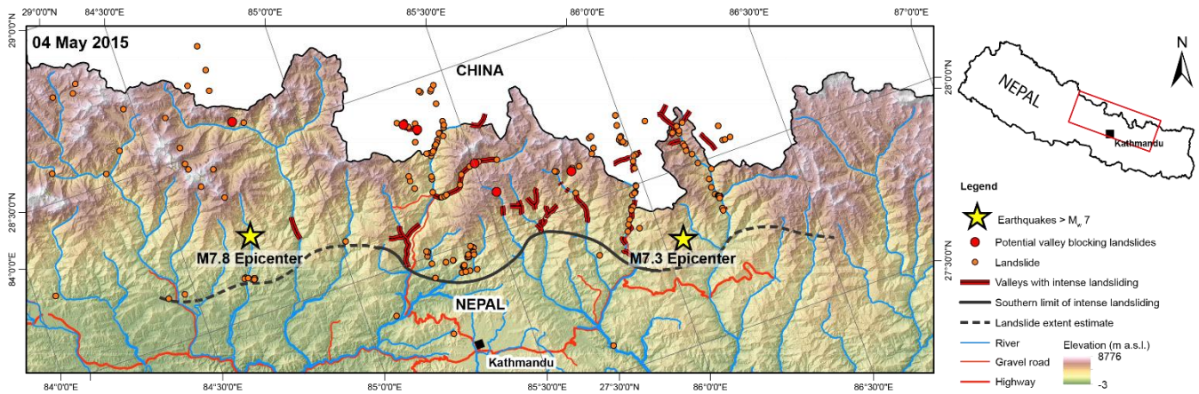
5 Figure 3: Extract from landslide impacts map released on 4 May 2015, nine days after the Gorkha earthquake and two days after cloud cover recession. Orange dots represent the location of observed individual landslides, at the point at which they reached the valley base. Red dots represent potential valley blocking landslides that had the potential to inhibit river flow, posing a future breach risk downstream. Red lines represent valleys identified as having experienced very intense landsliding, predominantly rockfall and dry debris flows. The black line delimited the southern limit of the area of intense landsliding. This limit was observed where solid and was anticipated where dashed, given that it was not visible in imagery. Both the 25 April (Gorkha) and 12 May (Dolakha) epicenters are added to this map for reference, despite its release prior to the Dolakha earthquake.
