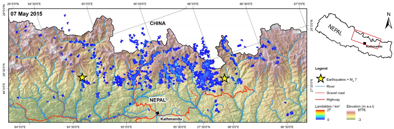
10 Figure 4: Extract from map released on 7 May 2015, 12 days after the Gorkha earthquake. Colored zone shows landslide distribution and relative intensity (number of landslides / km 2 ). The colour map has been adjusted to a range of 0-27 landslides / km 2 for comparison between Fig. 4-5. At this point, all areas in the map extent had been assessed using at least pan-sharpened Landsat 8 imagery (15 m). VHR (< 3 m) optical imagery had been used where available.
