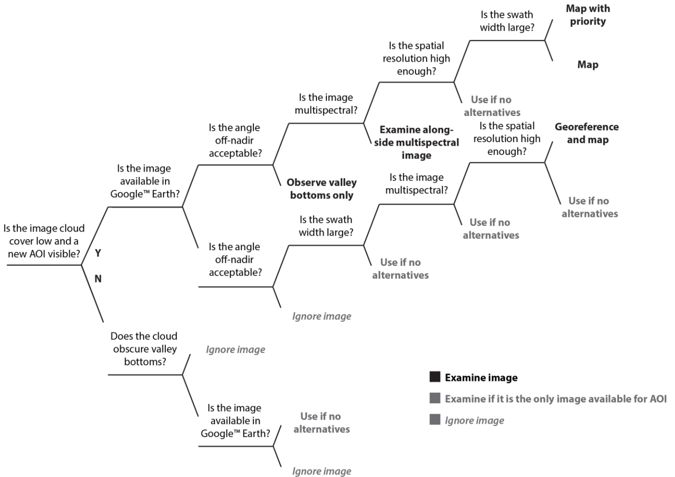
Figure 1. Decision tree for prioritising imagery used by Durham University for landslide mapping after the 2015 Gorkha earthquake. The relative importance of criteria decreases from left to right. Datasets were prioritized if they were efficient to pre-process and provided high-resolution data are optimal for mapping. Imagery with large swath widths and acceptable off-nadir angles may be difficult to acquire in mountainous terrain. These criteria were therefore prioritized to reduce the time spent georeferencing and the number of images required. Given the sub-metre resolution of VHR imagery and the ability to pan-sharpen multispectral imagery, most image resolutions are now sufficient to map landslides with the potential to cause significant damage. Spectral resolution was therefore considered as a more useful criterion for distinguishing landslides of this type than spatial resolution. This decision tree may also be applied to image selection for automated landslide mapping.
