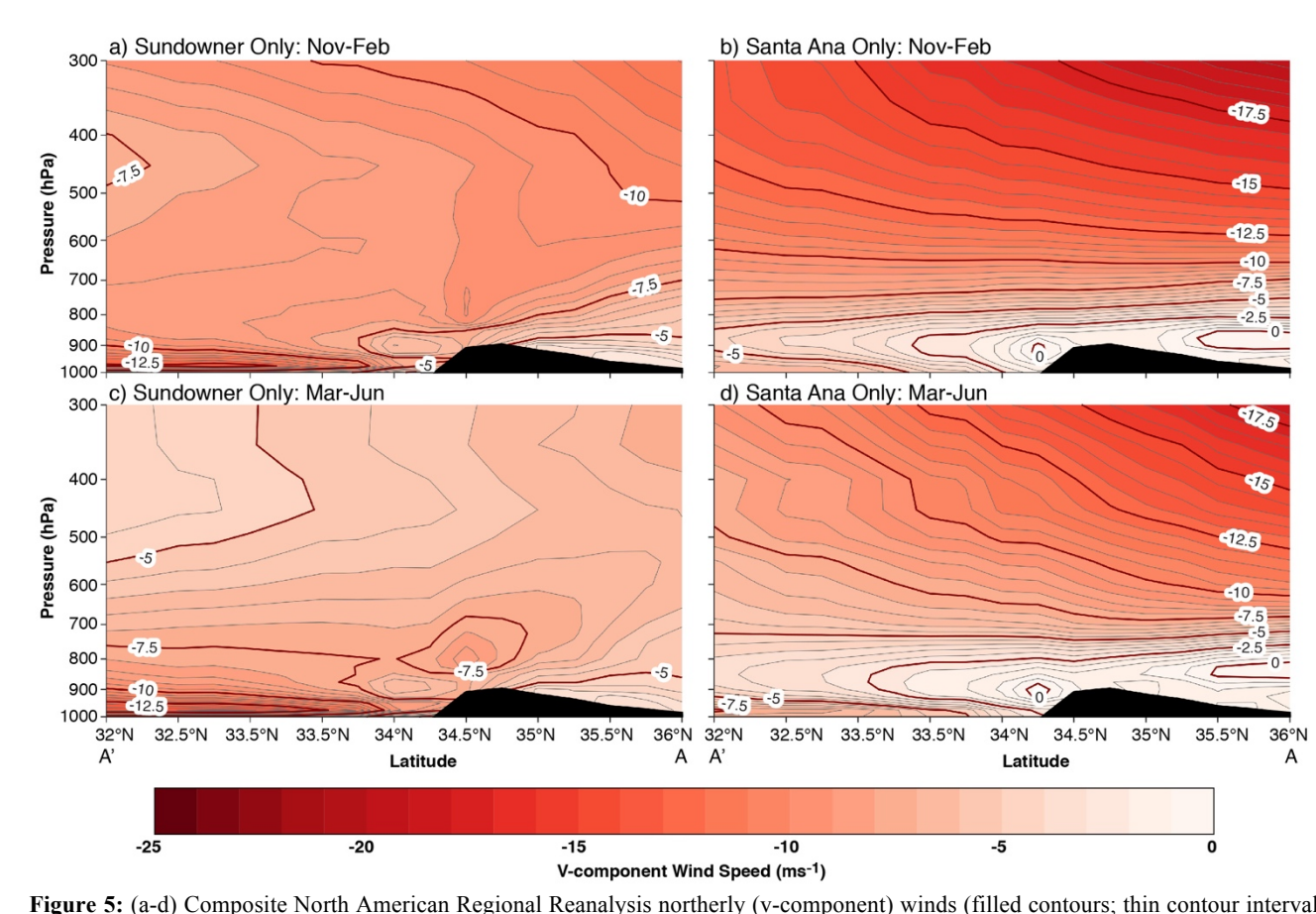
Figure 5: (a-d) Composite North American Regional Reanalysis northerly (v-component) winds (filled contours; thin contour interval 0.5 m/s; thick contour interval 2.5 m/s) for the cross-section spanning 32°N-36°N through the center of the study area longitude of 120°W. Black areas denote NARR terrain.
