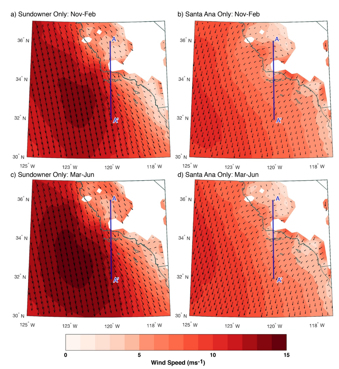
Figure 4: (a-d) Composite North American Regional Reanalysis 925 hPa wind velocity magnitude (filled contours, contour interval 1 \text{m s}^{-1} ) with vectors showing total wind direction (vector size is proportional to wind magnitude). Shaded white areas indicate areas where NARR terrain exceeds 925 hPa. The dark blue lines in each panel indicate the extent of the cross section used to produce the vertical cross sections shown in Figure 5.
