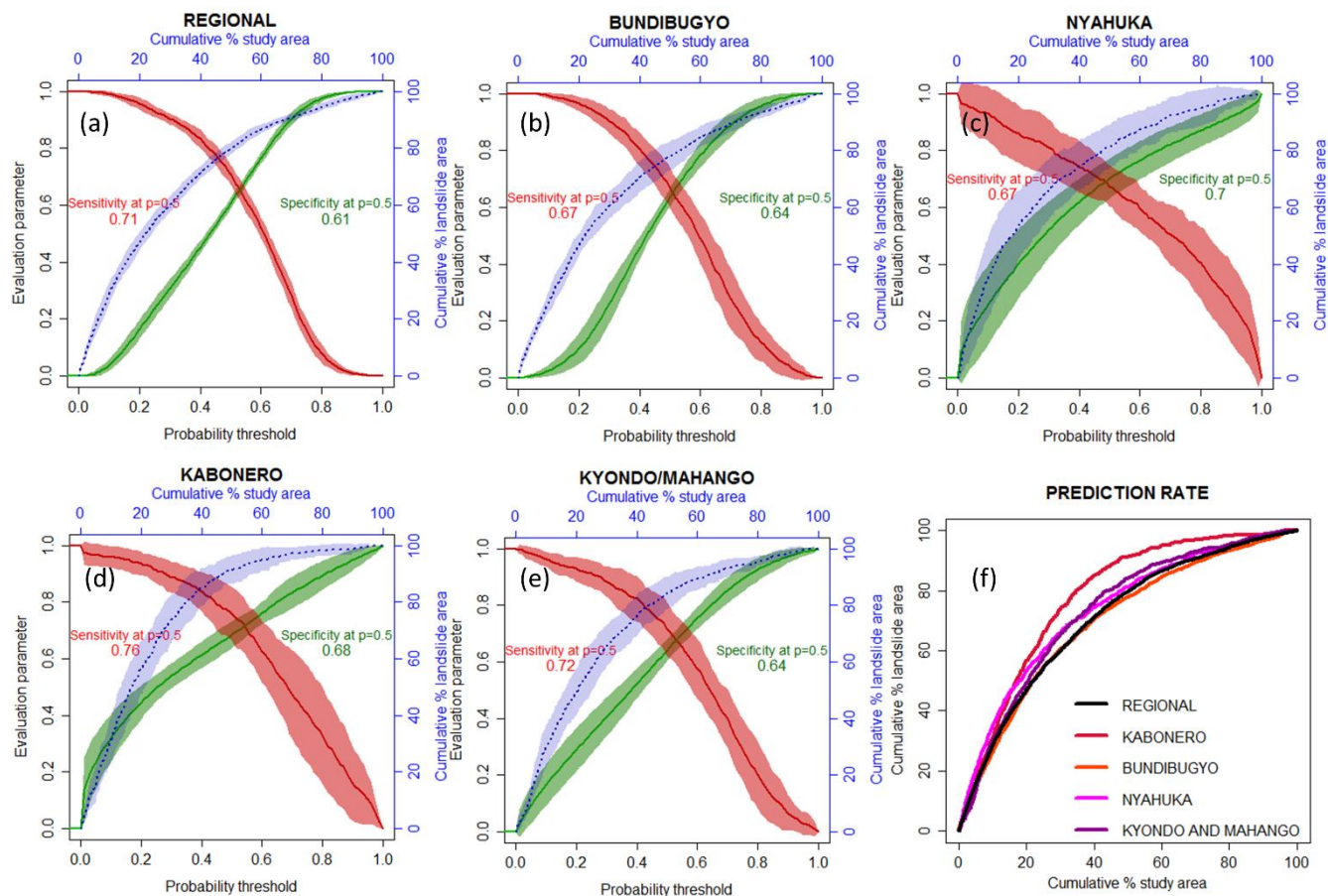
Figure 3: a to e: Sensitivity (red), specificity (green) and prediction rate curve (blue) of the selected model variants. Bold line represents the means and shaded areas the standard deviation of the metric over 20 simulations. f: mean prediction rates for selected models on the regional and local levels.
