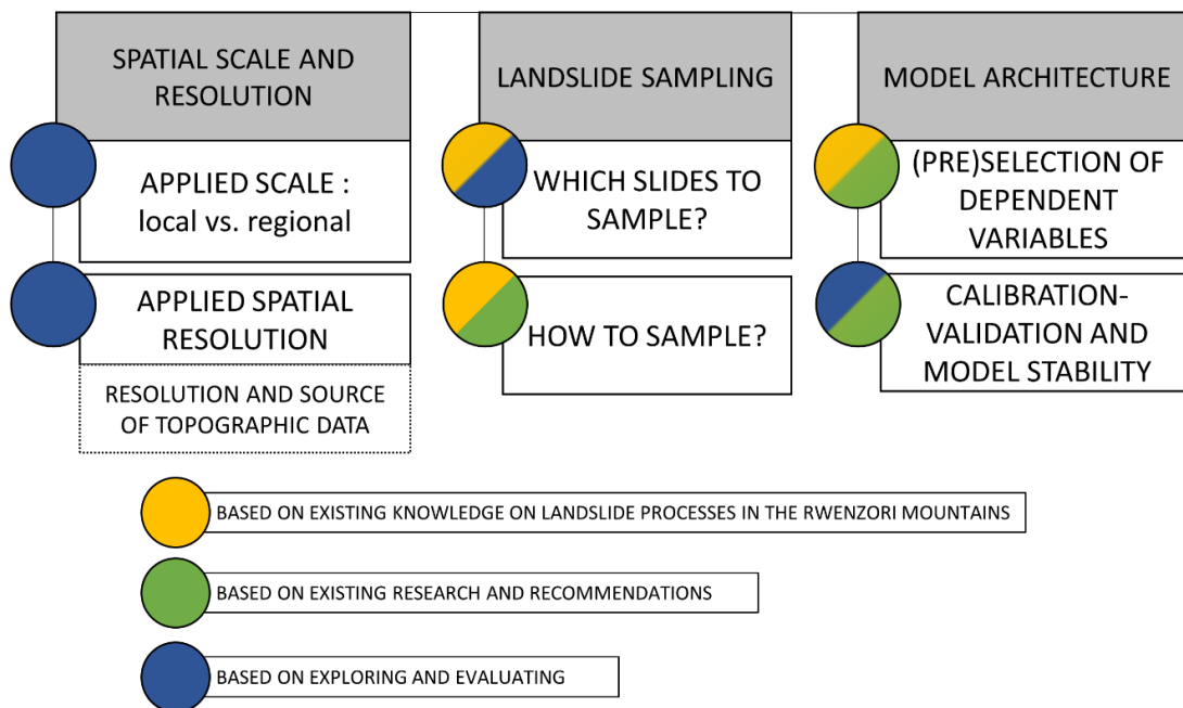
Figure 2: Schematic representation of the methodological options considered in this study and how they are evaluated and selected.
