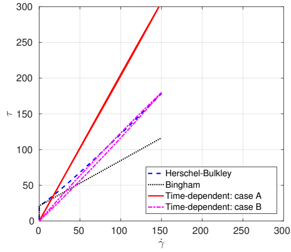
Figure 5. Analytical stress-strain for thixotropic avalanche Case 2: shear stress (Pa) and rate of strain (s ^{-1} ) with \tau_0 = 21.1 Pa and \tau_c = 165 Pa. The \tau axis is scaled for comparison with Figs. 4 and 6 while the \dot{\gamma} axis has an individual scale for clarity.
