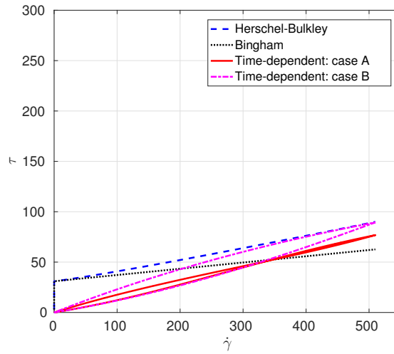
Figure 4. Analytical stress-strain for thixotropic avalanche Case 1: shear stress (Pa) and rate of strain ( s^{-1} ) with \tau_0 = 31 Pa and \tau_c = 90 Pa. The \tau axis is scaled for comparison with Figs. 5 and 6 while the \dot{\gamma} axis has an individual scale for clarity.
