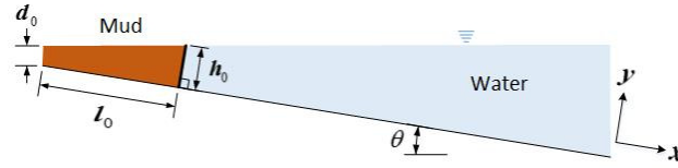
Figure 10. Schematic design of subaqueous debris flows
