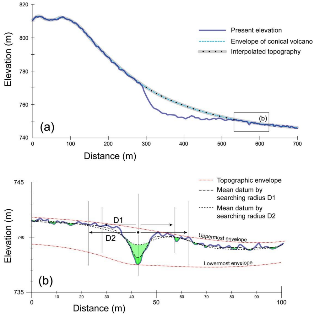
Fig. 9: Schematic illustration showing how the envelope of paleomorphology was obtained from the current DTM morphology. (a) The configurations of the undisturbed volcanic dome and current profile. The undisturbed volcanic dome facilitates the selection of manual interpolation points that better fit the volcanic edifice. (b) The configuration of the possible mean paleodatum correspondent to the other two enveloping surfaces. The shaded area represents the river incision. D1 and D2 correspond to different radii for topographic regression and restoration. The idealized profile was simplified and modified from a part of the topographic profile P4.
