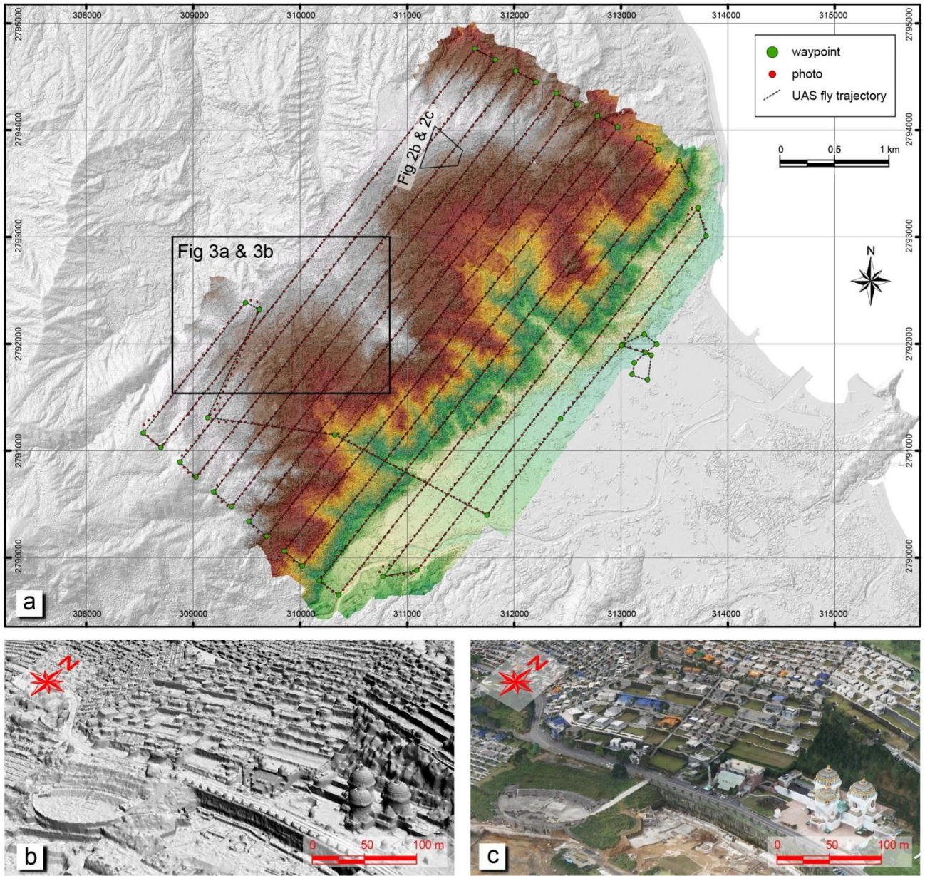
Fig. 2: Data acquisition from an unmanned aircraft system flight mission. (a) DSM generated by the UAS for a total area of 14.7 km 2 with a GSD of 6.6 cm, where points and lines represent the positions and path of the flight mission, respectively, and the monotone gray area is the LiDAR DSM; (b) side view of the hillshaded true 3D model; and (c) image draped onto the true 3D model. The side views of (b) and (c) are captured at the same position and orientation.
