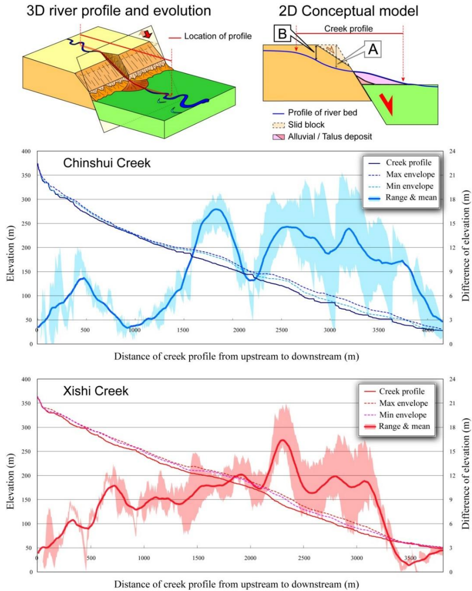
Fig. 12: River longitudinal profile and morphological evolution in the sliding area. Because of normal faulting, the substantial subsidence of the hanging wall led to a sudden reduction of the river bed. The block diagram shows the relationship between the river profile and normal faulting. The sharp fault scarp can be smoothed or even eroded by many small-scale landslides along the fault line. Therefore, the largest section of river incision may be located far from the fault scarp (marked as B), rather than close to the fault scarp (marked as A). The incision of creeks is obtained from the difference between the current and reconstructed profiles. The locations of the creek segments are shown in Fig. 11. The profile length has been normalized using the differences in the total length between the water source and basin mouth. The shaded bands form the error bar derived using different methods. The terrain elevation is extracted from LiDAR DTM.
