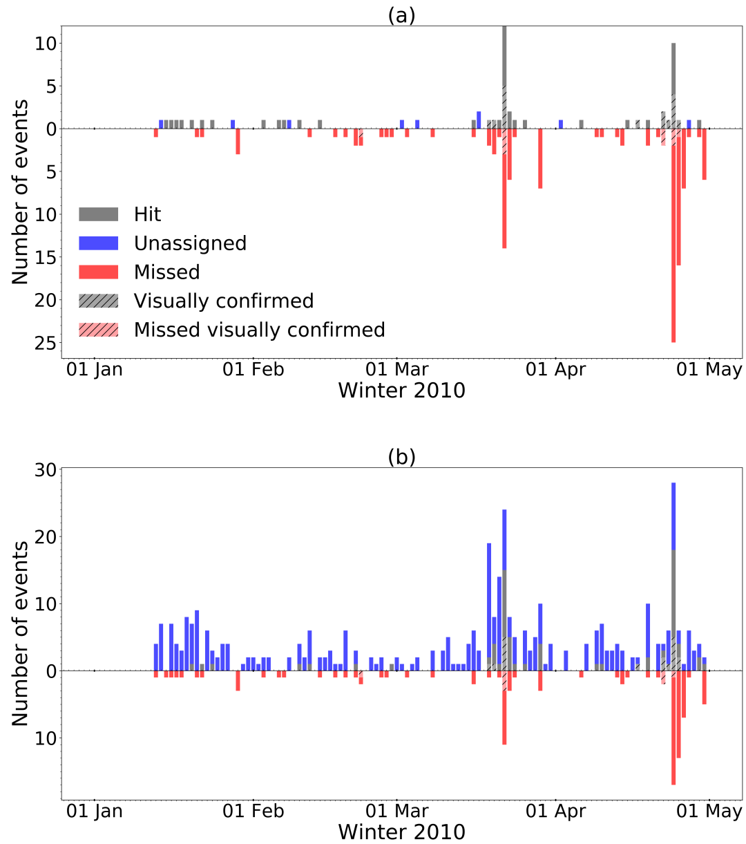
Figure 9. Classification results using a minimal event duration length of 12s for (a) sensor 1 and (b) sensor 7. Gray bars show the number of matching detections (hit), blue bars show the unassigned events and the red bars show the events that were not detected as an avalanche (missed). The hatched bars indicate the number of hits (grey) or misses (red) for the confirmed events.
