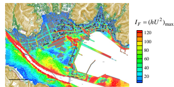
Fig. 20: I_F -value mapping for the original building array ( C = 0.01 ).
