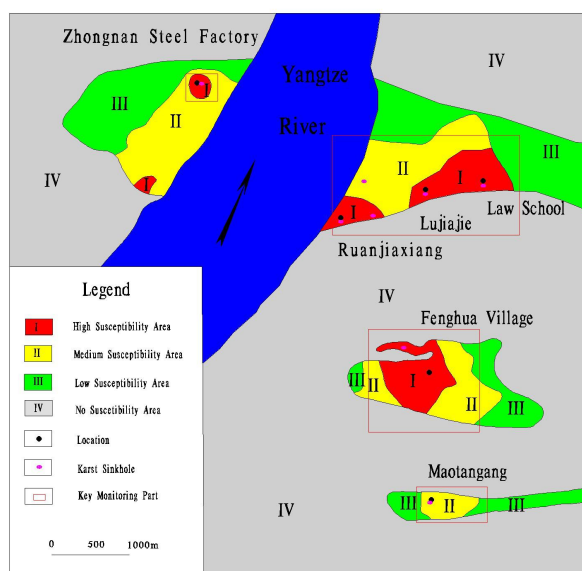
Fig.5.The risk distribution of karst collapse in Wuhan
