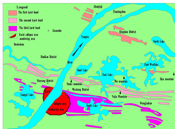
Fig. 4. Limestone distribution bands in Wuhan.
