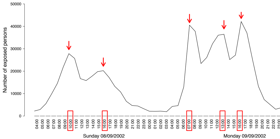
Figure 10: Temporal distribution of simulated traffic load at road cuts, which represent the hourly number of exposed persons. Results obtained by the simulation of MobRISK model for the 8-9 September 2002 flash flood event in the Alès study area (Gard).
