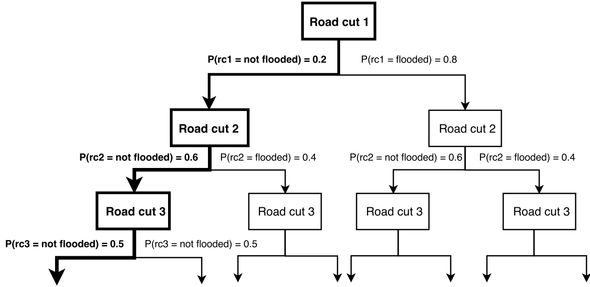
Figure 5: Probability tree diagram representing the method to measure motorists' flood risk exposure. The highlighted (bold lines) path represent the example of a motorist who crossed 3 road cuts ( rc ) with the following probabilities of submersion: P(rc_1 = 0.8) , P(rc_2 = 0.4) and P(rc_3 = 0.5) . His/her exposure is represented as a probability tree diagram where the nodes are the encountered road cuts and the arcs represent the probability of submersion in each road cut as shown in the Figure. First, we calculate the probability that the driver doesn't cross a flooded road cut that corresponds to the product of probability of not submersion in the crossed road cuts: P(\text{not submerged road cuts}) = (1 - P(rc_1)) * (1 - P(rc_2)) * (1 - P(rc_3)) = 0.06 . Then, final exposure corresponds to: 1 - P(\text{not submerged road cuts}) = 0.94 .
