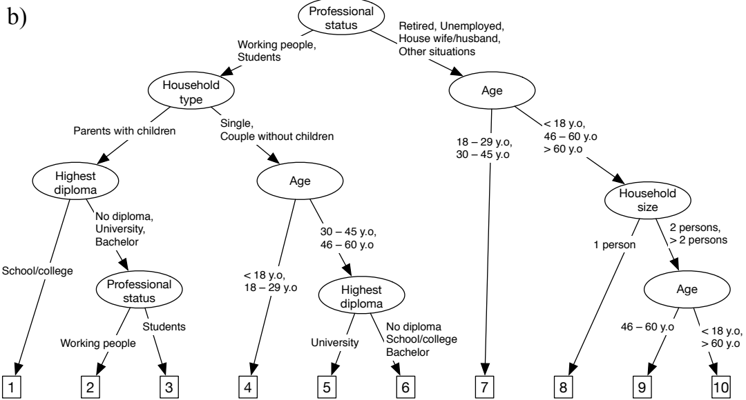
Figure 6: Regression tree results for weekday schedules (a) and weekend schedules (b) indicating respectively 12 and 10 clusters of schedules respectively. The upper part of the figure displays the regression tree is displayed: each node represents the variable splitting the schedules into 2 groups and each arc represents the group/category. A visual representation of the weekday schedules corresponding to each cluster is displayed at the bottom of 6a: each activity is represented by a color and each line is representing a sequence of activities.
