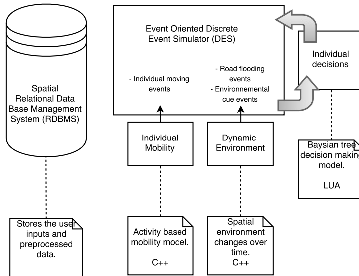
5 Figure 1: MobRISK model architecture includes: (i) the simulated environmental changes considered for the study such as roads' flooding; (ii) an activity based mobility model reproducing population travel-activity behaviors; (iii) a decision-making model predicting individual responses to weather disruptions. A Discrete Event Simulator (DES) rules the main temporal loop of the simulations. In addition, the user input data is stored in a spatial relational database management system.
