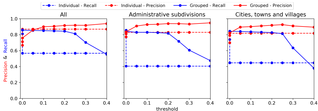
Fig. 2. Recall and precision scores for individual and grouped geoparsing with a varying threshold.
