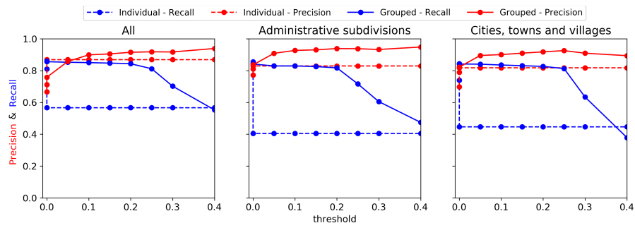
Fig. 2. Recall and precision scores for individual and grouped geoparsing with a varying threshold.
