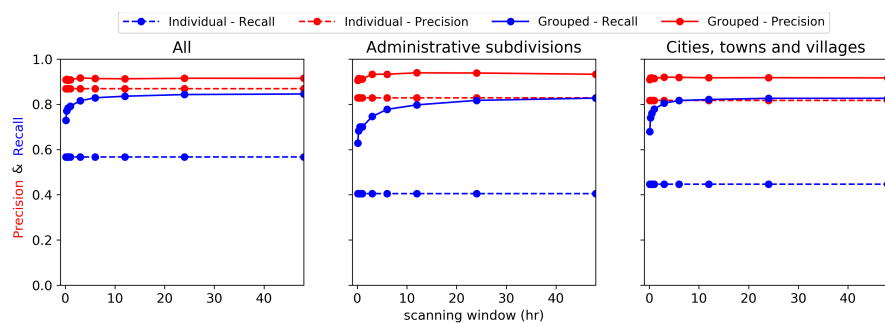
Fig. 1. Recall and precision scores for individual and grouped geoparsing with a varying size of the scanning window.
