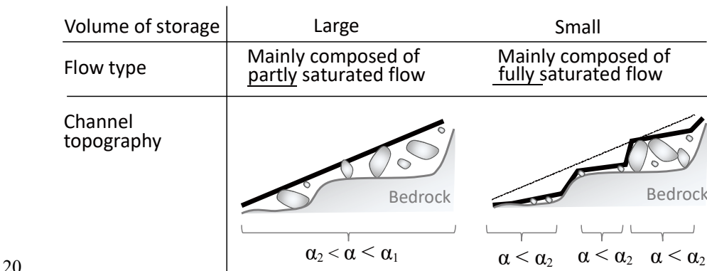
Figure 12: Schematic diagram of the relationships between the volume of storage, flow type, and channel topography. \alpha is the channel gradient, \alpha_1 is the theoretical boundary of the channel gradient between fully unsaturated and partly saturated sediment transport, and \alpha_2 is the theoretical boundary of the channel gradient between partly and fully saturated sediment transport.
