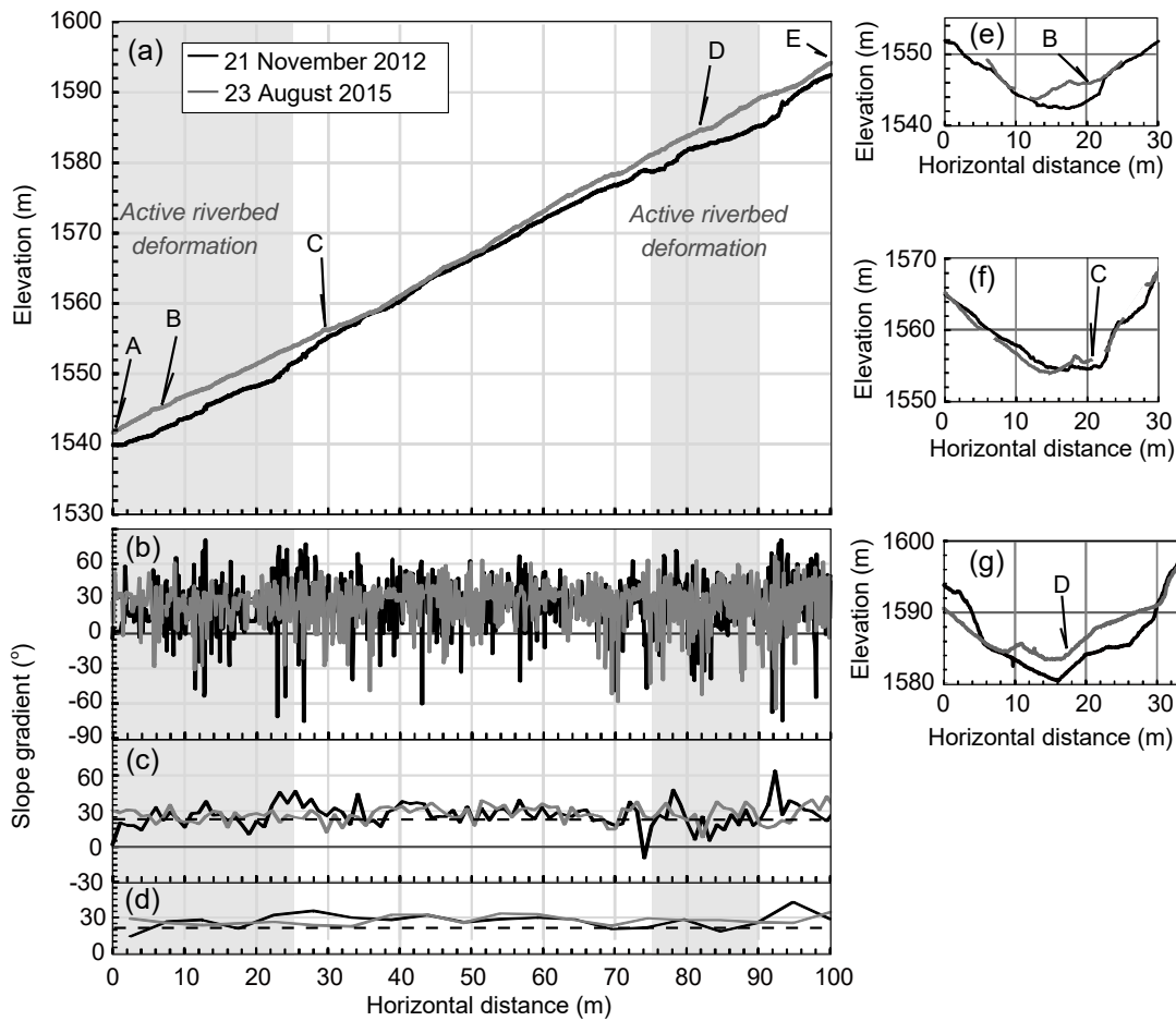
Figure 10: Channel profiles and channel gradient mainly formed by fully saturated flow (measured on 21 November 2012 after the debris flow on 30 September 2012) and partly saturated flow (measured on 23 August 2015 after the debris flow on 6 August 2015), obtained from 0.1 m terrestrial laser scanning (TLS) derived digital elevation maps (DEMs). (a) Longitudinal channel profile in the section between A to E in Fig. 2. (b) Longitudinal changes in the channel gradient calculated for each section with a length of 0.1 m. (c) Longitudinal changes in the channel gradient calculated for each section with a length of 1.0 m. (d) Longitudinal changes in the channel gradient calculated for each section with a length of 5.0 m. (e) Cross-sectional profile of the channel at point B. (f) Cross-sectional profile of the channel at point C. (g) Cross-sectional profile of the channel at point D. Data at some cross-sections on 9 August 2015, are absent because of the failure of the TLS survey due to the weather conditions (panels e and f).
