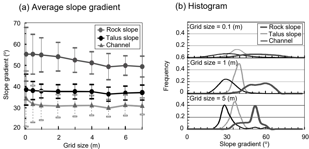
Figure 9: Slope gradient of typical geomorphic units calculated from terrestrial laser scanning (TLS) derived digital elevation maps (DEMs) with various grid sizes. Topographic data in all measurement periods were used in the statistical analysis. (a) Changes in the average slope gradient of each geomorphic unit with an increase in the grid size. The slope gradient in all periods was averaged. The bars attached to the plots indicate the range of the standard deviation. (b) Histogram of the slope gradient calculated from TLS DEMs, with grid sizes of 0.1, 1.0, and 5.0 m. Integrals of the frequency for each geomorphic unit in Fig. 8b, which are categorized with 2 degree step, are all 1.
