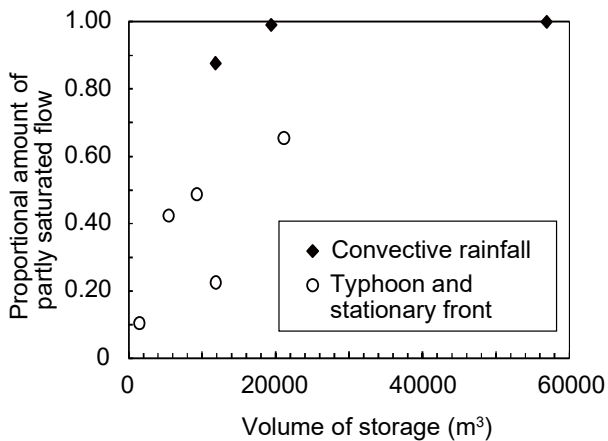
5 Figure 7: Comparison between the volume of storage and the duration of partly saturated flow as a proportion of the overall debris flow surges. Rainfall duration and total rainfall depth of the convective rainfall are <5 h, and <50 mm respectively, while those of typhoon and stationary fronts are >5 h, and >50 mm respectively.
