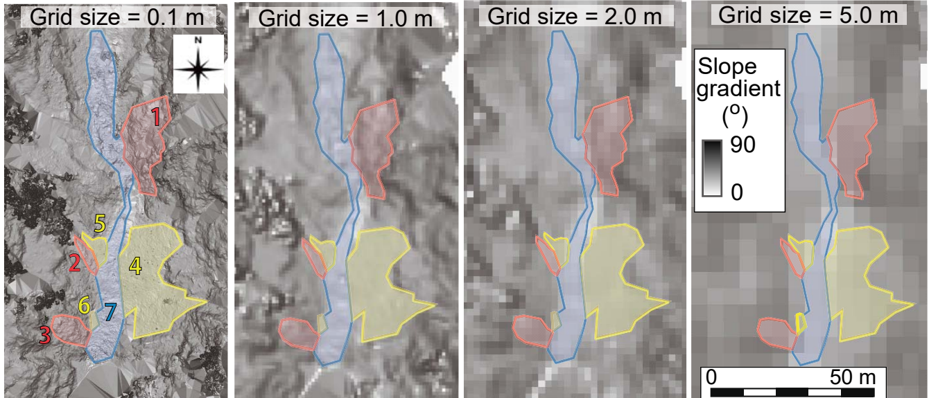
10 Figure 8: Slope gradient map calculated after using terrestrial laser scanning (TLS) data on 14 May 2014, with various grid sizes. The location of the analysis area is shown in Fig. 2. Areas colored red, yellow, and blue indicate rock slopes, talus slopes, and a channel, respectively
