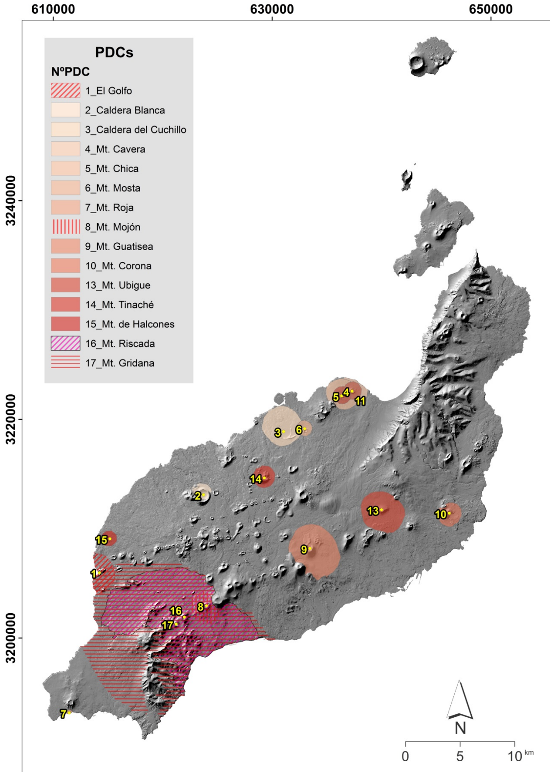
Figure 7. PDC scenarios performed with VORIS 2.0.1. Covered areas with different collapse equivalent heights ( H_c ) and collapse equivalent angles ( \theta ) (see the text for more detail). Different symbols (dashed, filled and coloured) have been used to show the limits of each PDC. Yellow dots indicate the simulation starting point.
