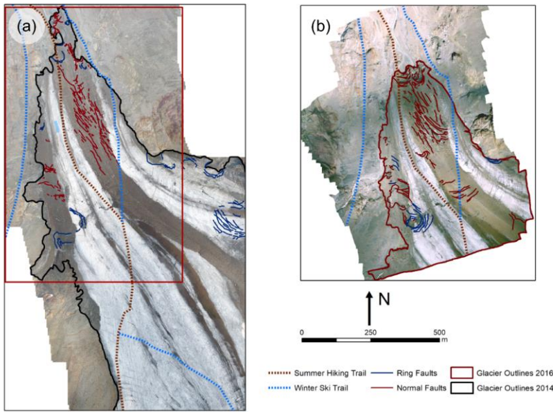
Figure 7: Location of collapse structures, i.e. normal faults and ring faults and trails crossing the Forni Glacier. (a) Collapse structures in 2014, with 2014 UAV orthophoto as basemap. The red box marks the area surveyed in 2016. (b) Collapse structures in 2016, with 2016 UAV orthophoto as basemap. Trails from Kompass online cartography at https://www.kompass-1039 italia.it/info/mappa-online/ .
