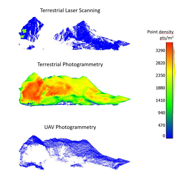
Figure 5: Maps of point density in sample location 2.
