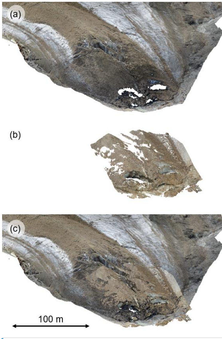
Figure 6: Spatial coverage of UAV- and terrestrial photogrammetry point clouds and merged point cloud from the two techniques. a) UAV photogrammetry point cloud; b) terrestrial photogrammetry point cloud; c) merged point cloud.
