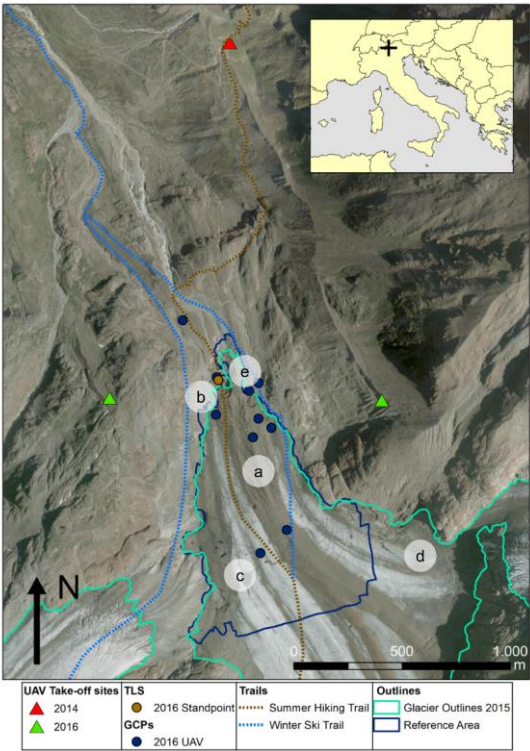
Figure 1: the tongue of Forni Glacier. The map shows the location of take-off/landing sites for the 2014 and 2016 UAV surveys, standpoint of TLS survey, GCPs used in the UAV photogrammetry surveys and trails crossing the glaciers. Letters a-e identify the location of features described in Fig.2. Base map from 2015 courtesy of IIT Regione Lombardia WMS Service. Trails from Kompass online cartography at https://www.kompass-1039italia.it/info/mappa-online/ .
