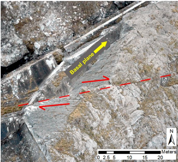
Figure 12. Detail of the zenithal orthophoto with indication of apparent motion of a major fault acting as back release surface for block A of figure 9.
