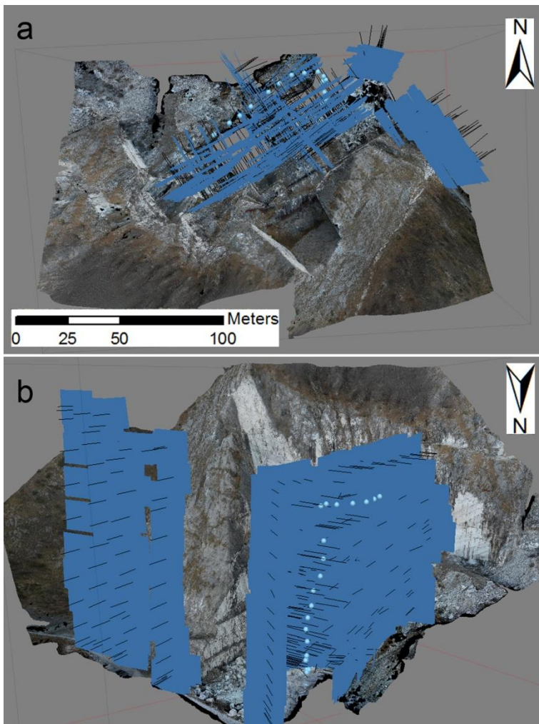
Figure 5. Plan view (a) and perspective view (b) of the RPAS frontal surveys (blue rectangles correspond to the photographs locations, black lines to normals). Corresponding 3D point cloud produced with photogrammetric processing of digital images is shown in background.
