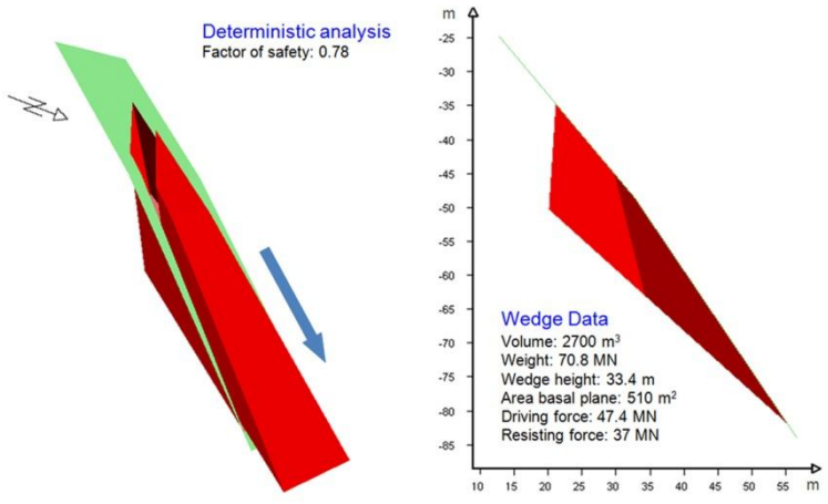
5 Figure 10. Result of Swedge 3D preliminary slope stability analysis.
