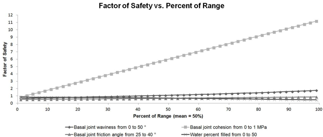
5 Figure 11. Result of sensitivity analysis relative to basal joint waviness, friction angle, cohesion and water percent filled parameters.
