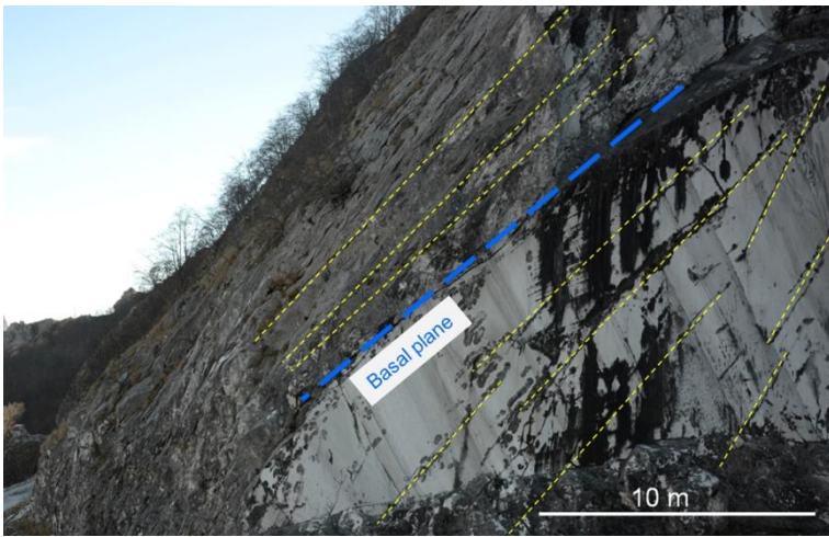
Figure 13. Details of a series of high discontinuities over and below the basal plane under study.
