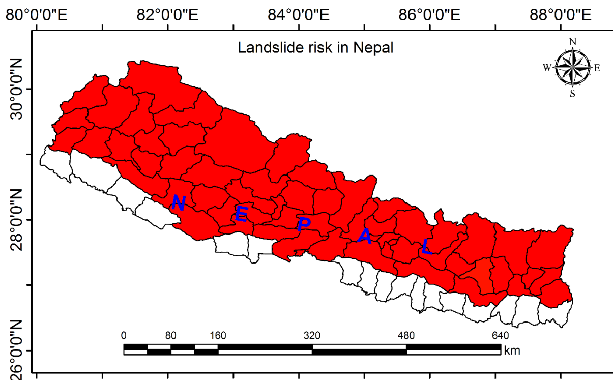
Fig. 2 Generalized landslide risk map for Nepal
