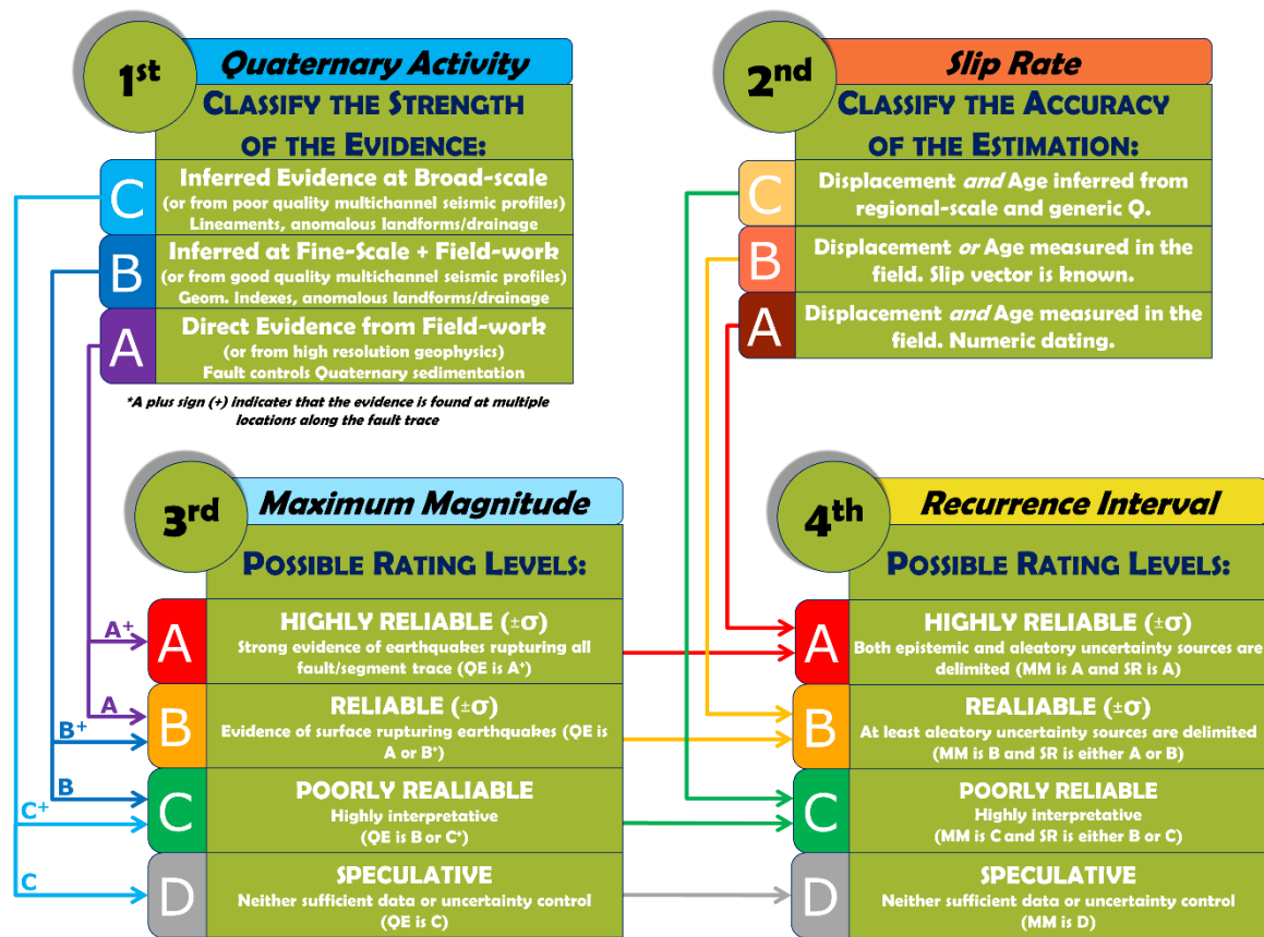
Figure 4. Diagram summarizing the scheme followed in QAFI v.3 for rating the reliability of Maximum Magnitude (RMM) and Recurrence Interval (RRI) on the base of the Strength of the Quaternary activity Evidence (SQE) and the Accuracy of the Slip Rate estimation (ASR). First, the SQE of the fault is classified based on the detail of the available published observations in three increasing levels of accumulated evidence, varying from C (weak) to A (very strong). A plus sign (+) is assigned when the observations can be extrapolated with confidence all along the fault trace. Second, the ASR is classified based on the accuracy of the information used for its determination, varying from C (rough) to A (accurate). Third, RMM is obtained from SQE class, varying from A (Highly Reliable) to D (Speculative). Fourth, RRI is obtained from both RMM and ASR. The resulting RRI would never be higher than the rated level for RMM, yet it could be lower depending on the ASR (these relationships are not shown on the diagram for the sake of simplicity). See text and Table 1 for a more extensive explanation.
