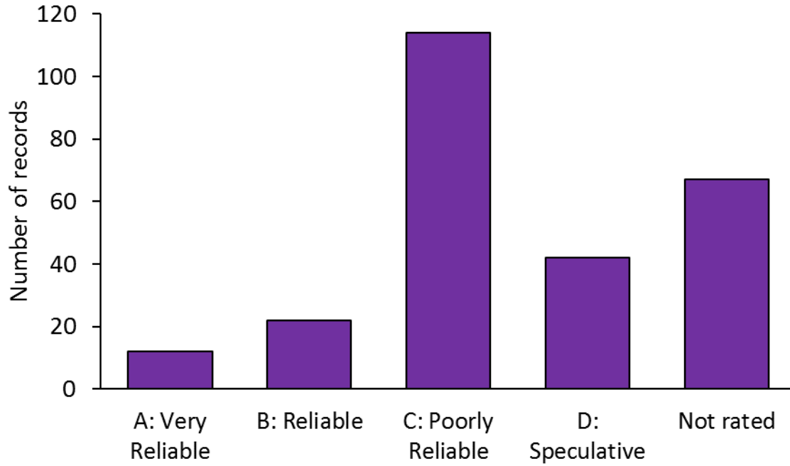
Figure 6. Distribution of rating levels for the database-field Reliability of Recurrence Interval (RRI) in QAFI v.3 database. See text for explanations.
