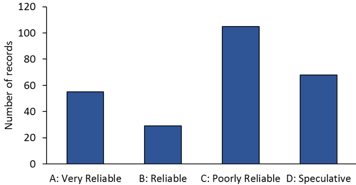
Figure 5. Distribution of rating levels for the database-field Reliability of the Maximum Magnitude estimation (RMM) in QAFI v.3 database. See text for explanations.
