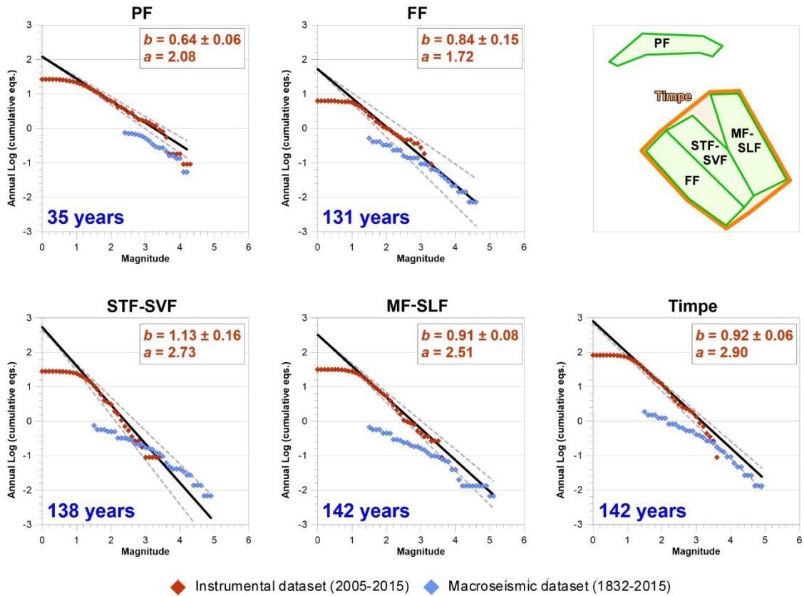
670 Figure 6: Frequency Magnitude Distribution for each SZ. Red dots refer to the instrumental dataset, blue dots to the macroseismic one; dotted lines indicate uncertainties concerning the GR relationship (black line). b - and a -values are obtained from the instrumental earthquake dataset. Years indicate the actual time-window ( T_{\text{last}}-T_{\text{first}} ) of the events in each sub-catalogue of the historical dataset. Data are normalized to one year. Abbreviations as in Fig. 4.
