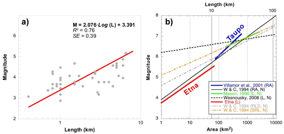
695 Figure 10: a) Plot of earthquake magnitude vs rupture length for the Etna region (this study); b) Comparison with the magnitude-size scaling relationships for the Taupo volcanic zone (Villamor et al., 2001) and other relationships worldwide (Wells and Coppersmith, 1994; Mason, 1996; Wesnousky, 2008). Abbreviations: L, fault length; N, normal kinematics; RA, rupture area; RLD, rupture length at depth; SRL, surface rupture length.
